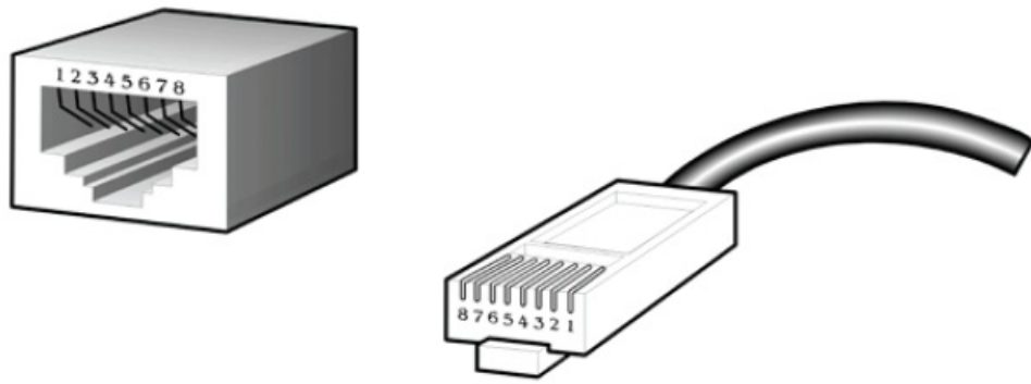
Figure 5 - RJ45 PoH Pin Assignment
