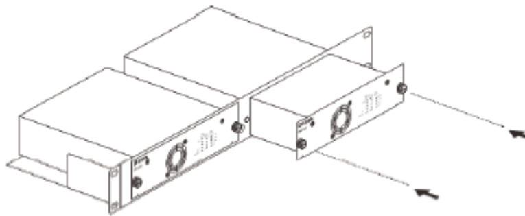
Figure 2 - Installing the DPS-520 into the DPS-800
