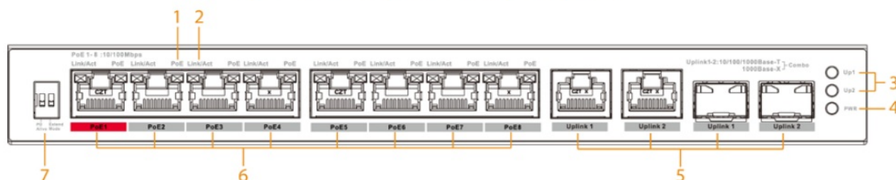
Figure 2-1 Front panel (with optical ports)
