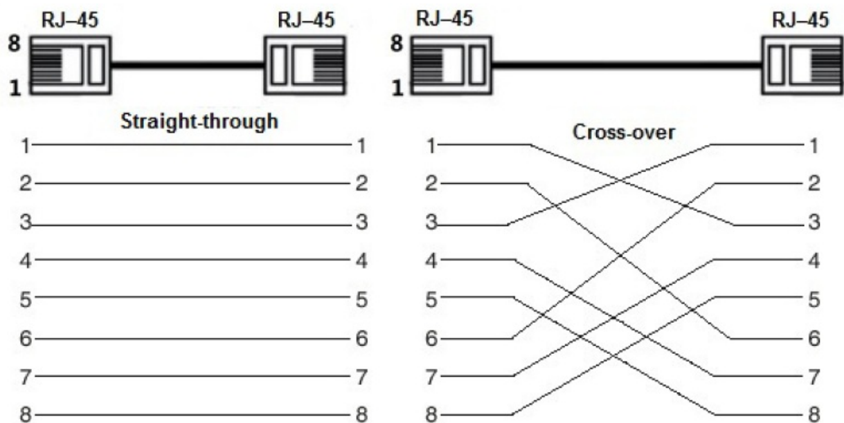
Figure 4-5 Pin description
