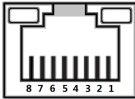
Figure 4-5 Pin description
