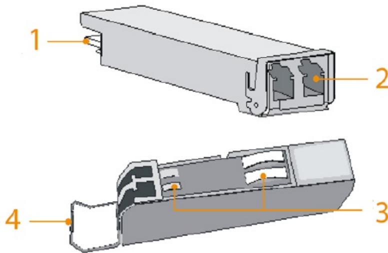
Figure 4-2 SFP module structure
