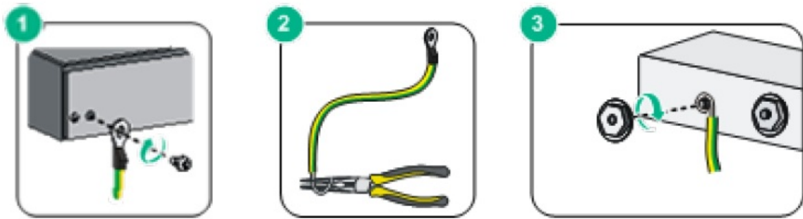
Figure 4-1 Connect GND
