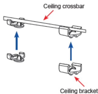
Figure 7: Attaching the Ceiling Brackets
