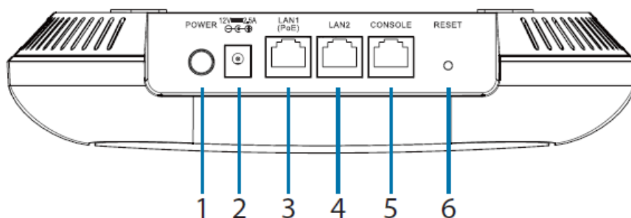
Figure 2: Rear Connectors
