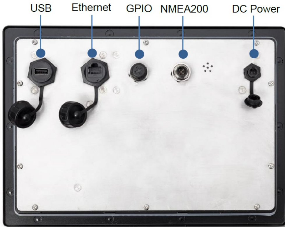
Figure 2. Touch 10 Rear
