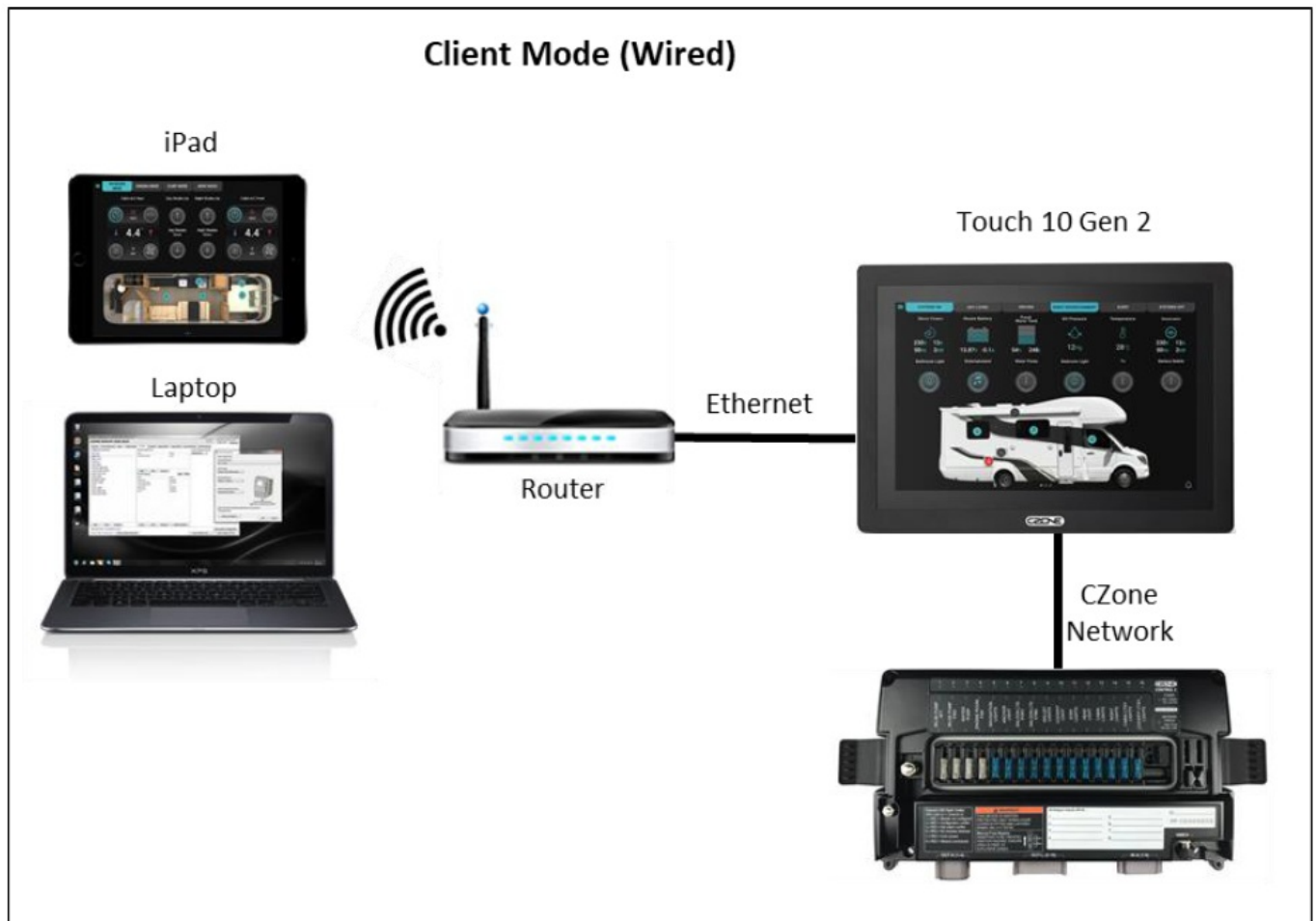
Figure 3. Client Mode Wired Example
