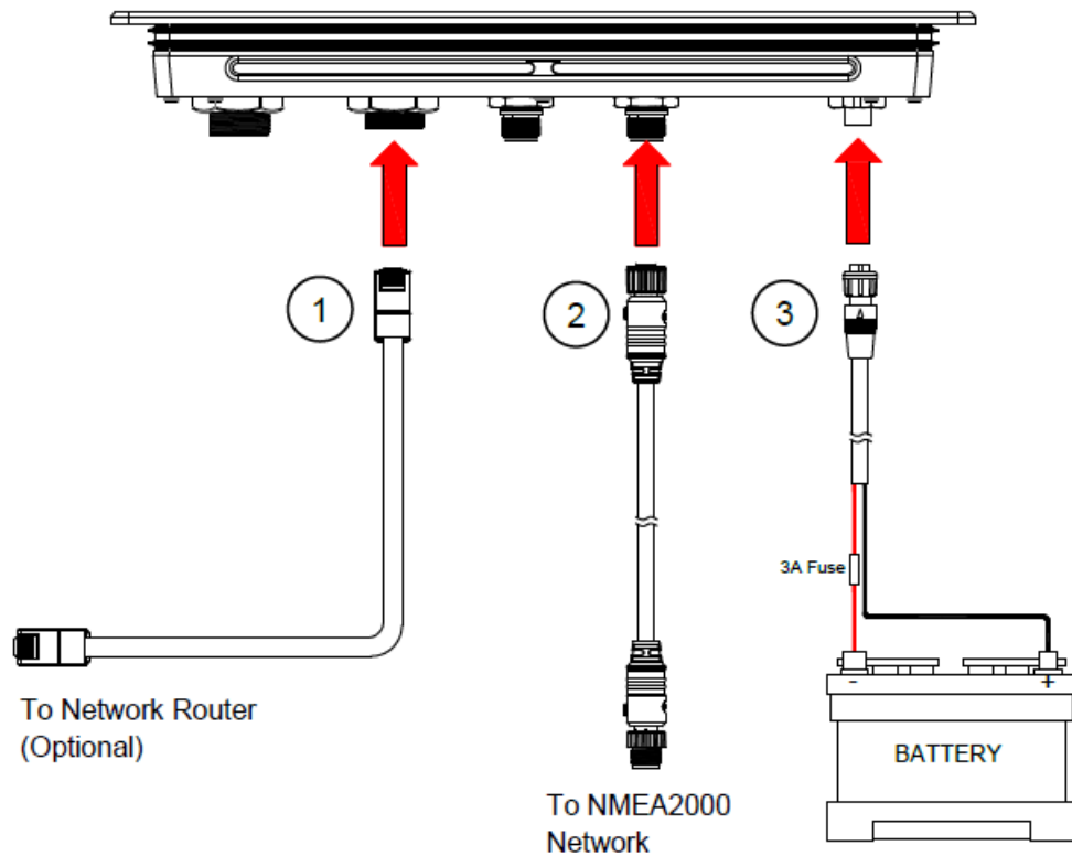
Figure 5. Connections
