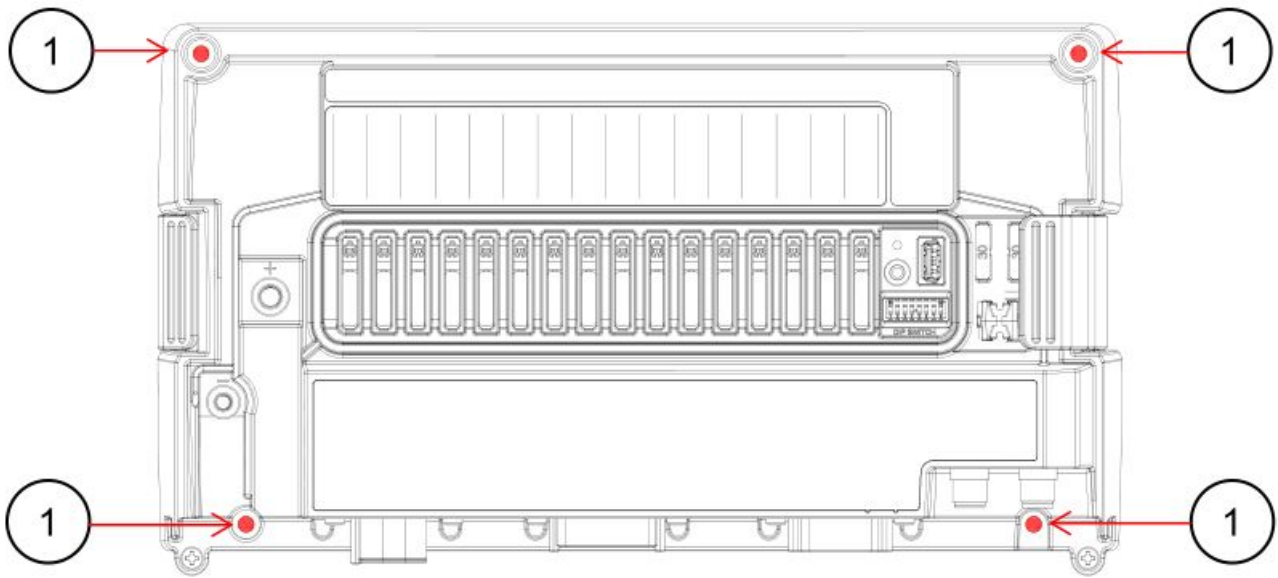
Figure 11. Mounting Screw Locations
