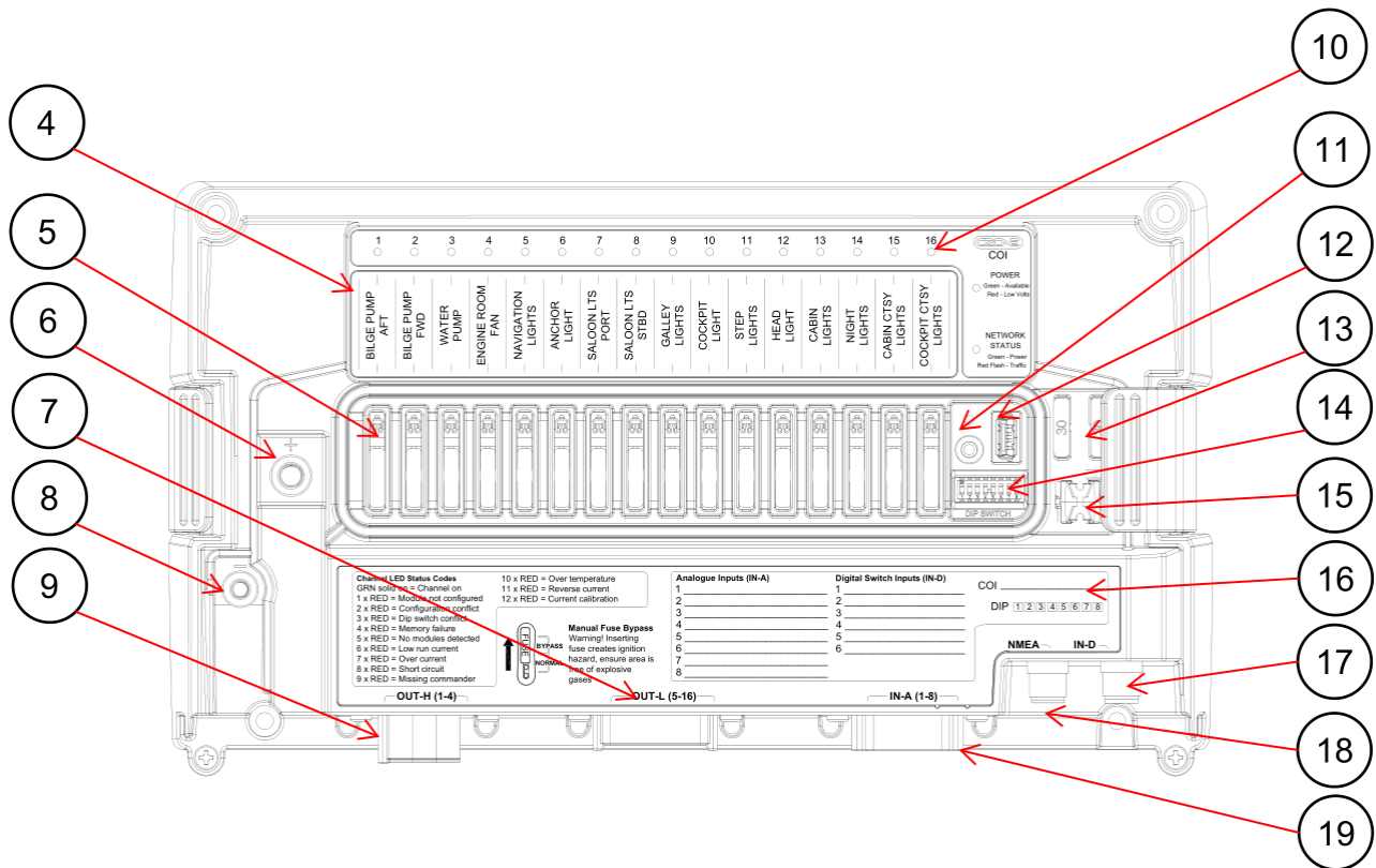
Figure 2. COI no covers
