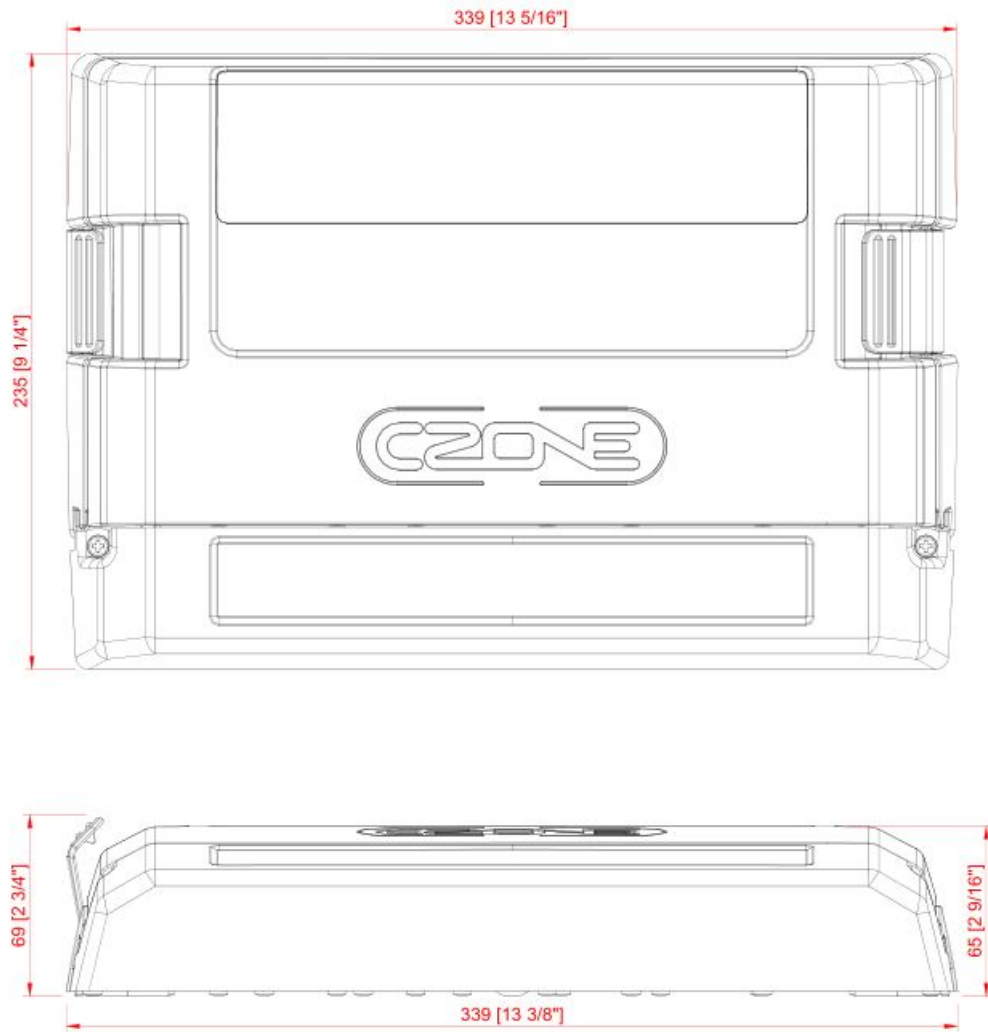
Figure 17. COI Dimensions with covers
