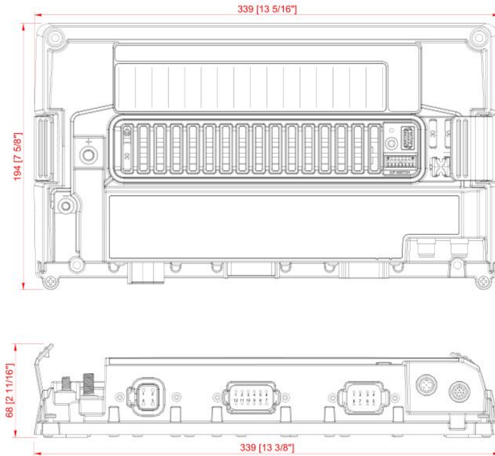
Figure 16. COI Dimensions no covers
