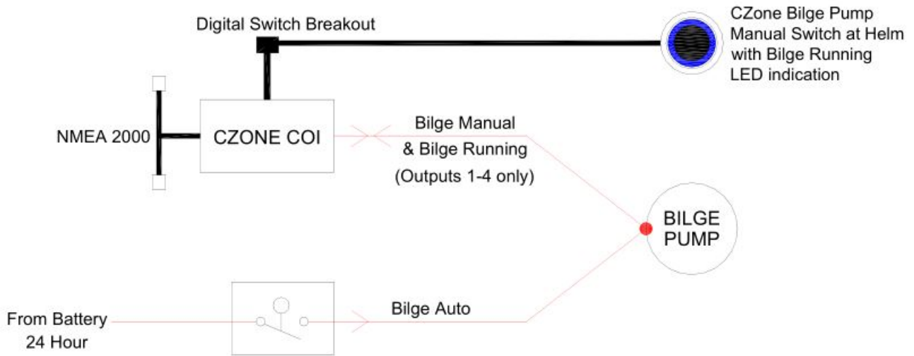
Figure 9. COI Bilge Pump Wiring Example
