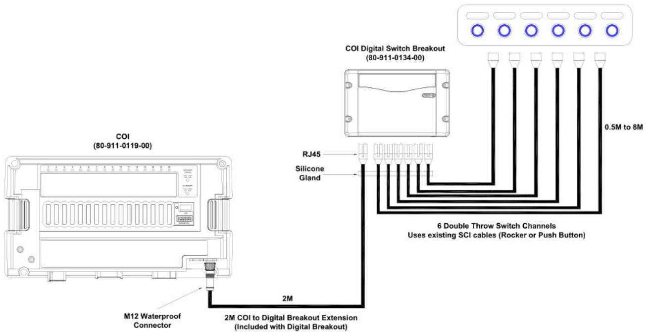
Figure 13. COI Digital Switch Breakout Connections
