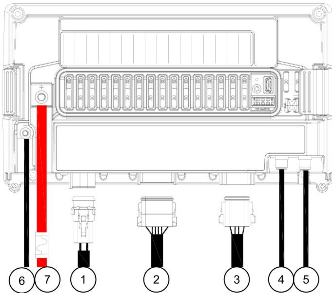
Figure 12. COI Connections
