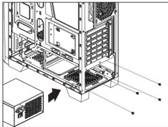
Install PSU
