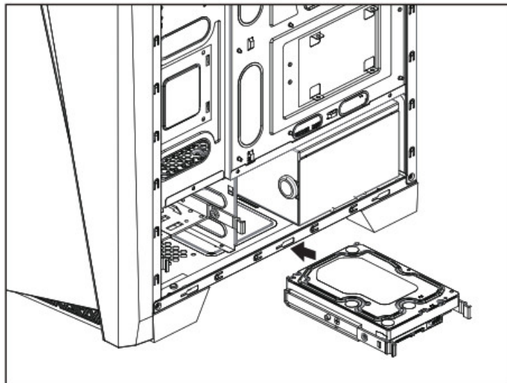
Install 3.5" HOD
