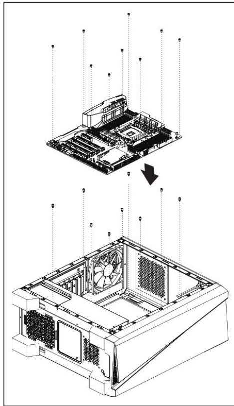
Install Motherboard
