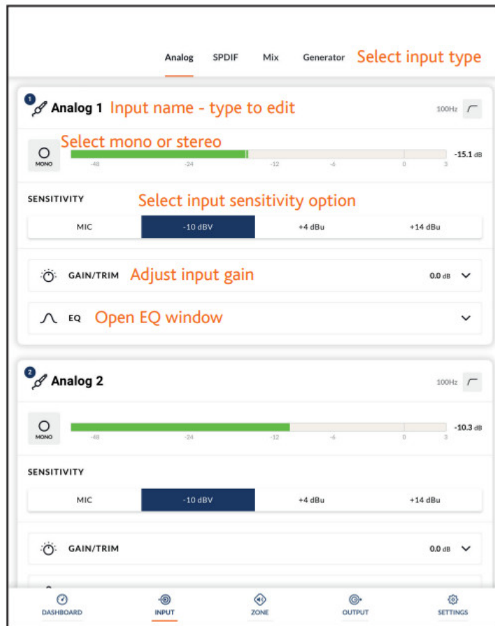
Diagram 5B Input Tab display (two inputs only shown)
