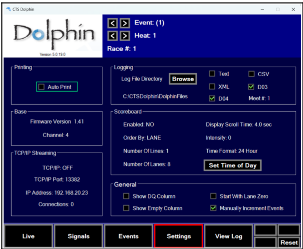
Figure 8: The CTS Dolphin Settings screen
