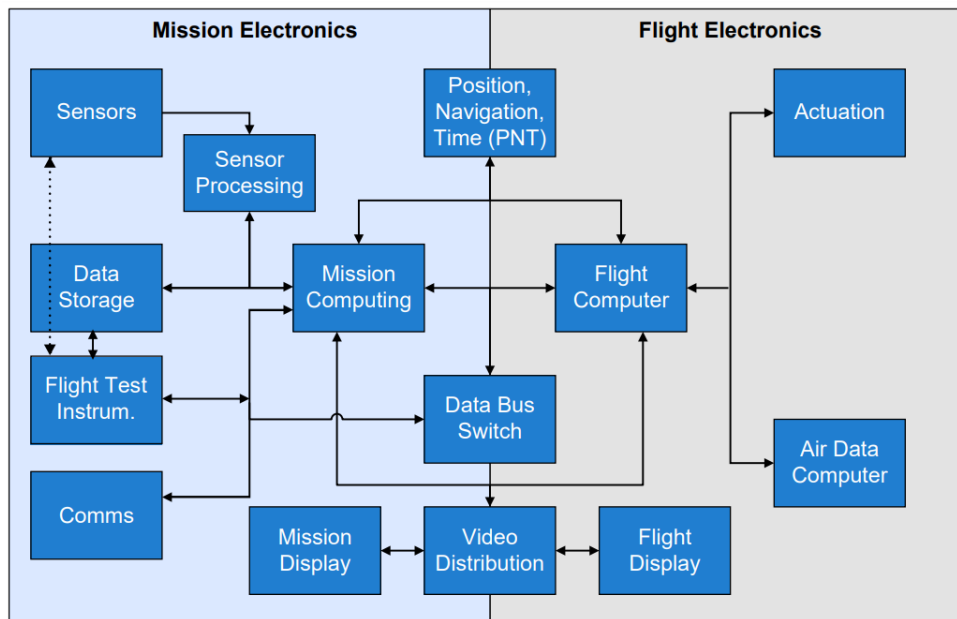
Generic airborne platform architecture
