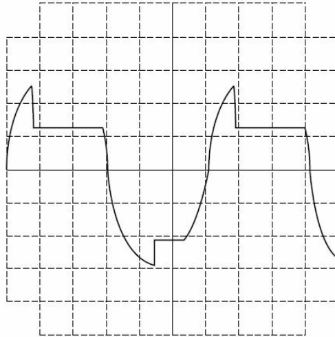
Figure 5. ODEP Limiting Wave Form
