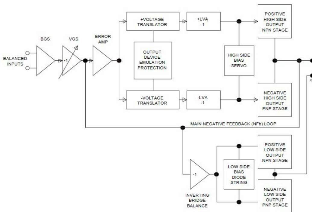
Figure 3. Typical Crown Amplifier Basic Block Diagram (One Channel Shown)
