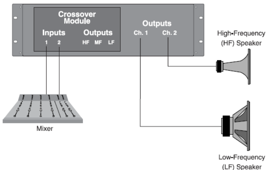
Figure 1.28 Typical Two-Amp, Bridge-Mono, Two-Way Hookup
