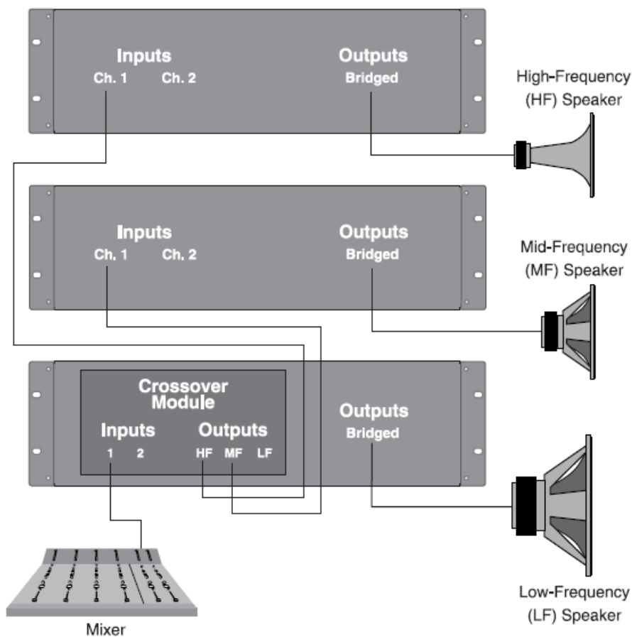
Figure 1.29 Typical Three-Amp, Bridge-Mono, Three-Way Hookup
