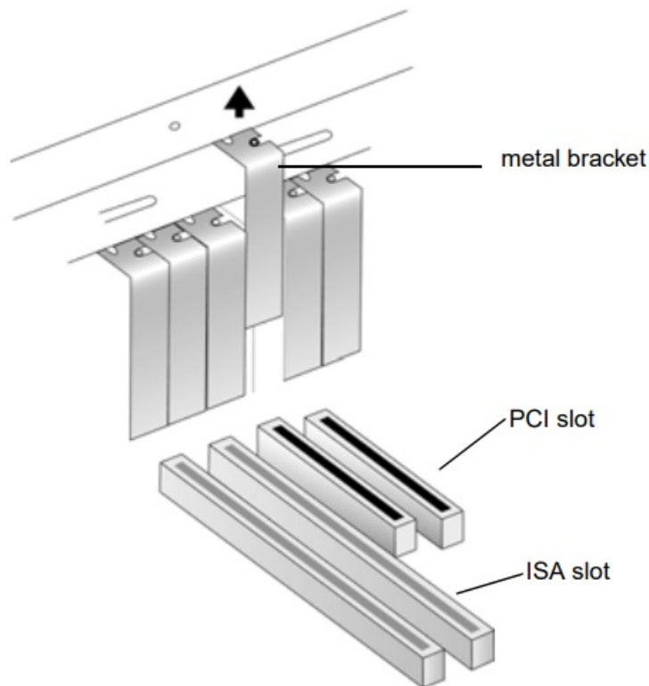
Figure 1-2: Removing a metal bracket.
