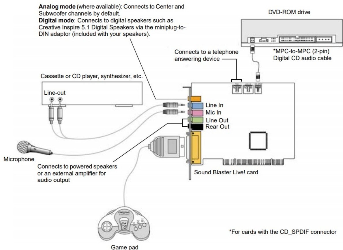
Figure 1-5: Connecting Sound Blaster Live! to other devices.
