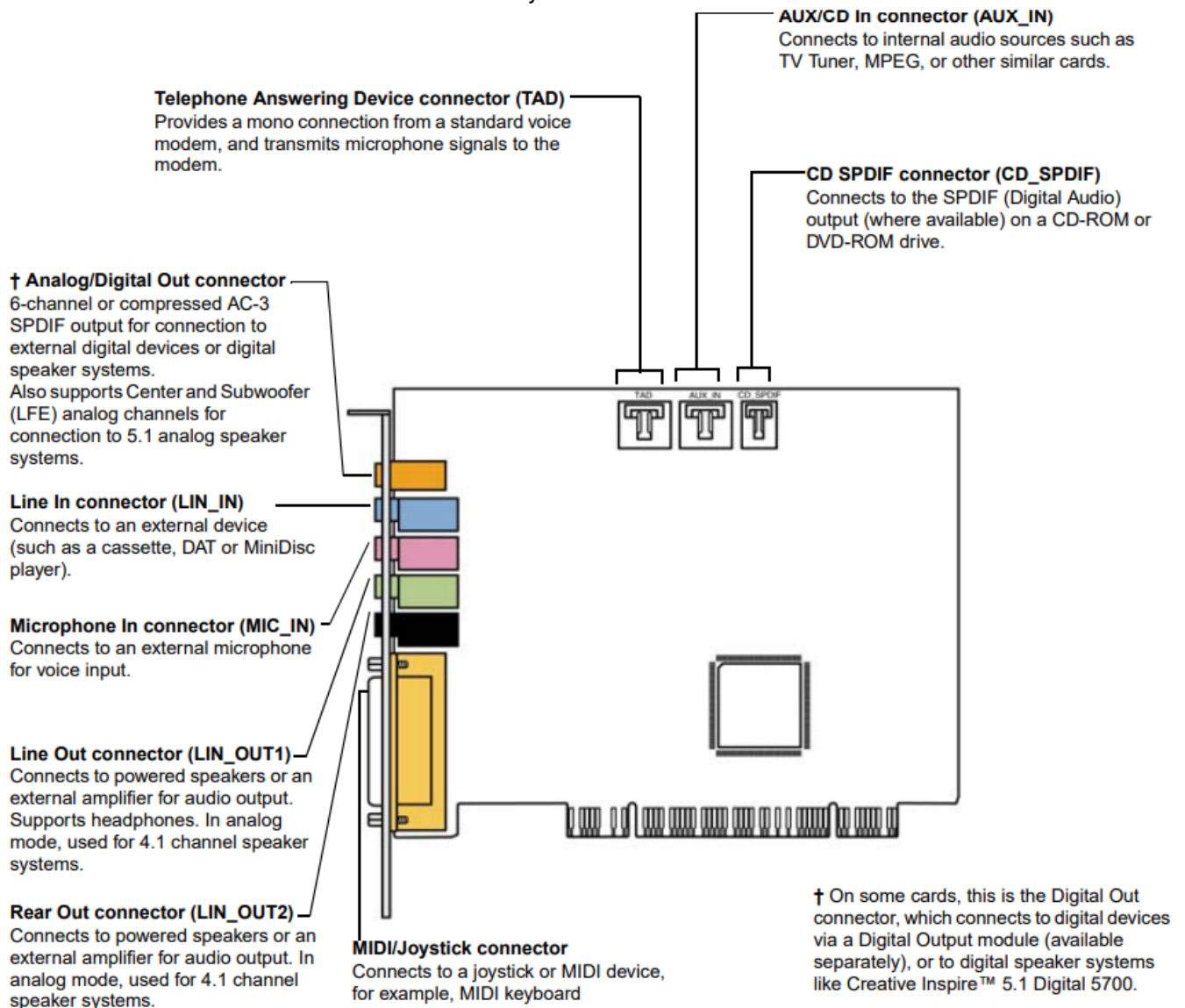
Figure 1-1: Connectors on the Sound Blaster Live! card.
