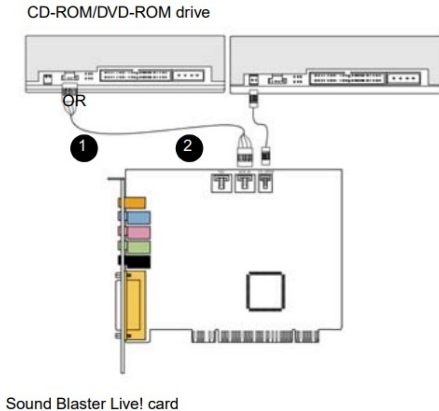
Figure 1-4: Connecting CD-ROM/DVD-ROM drives.
