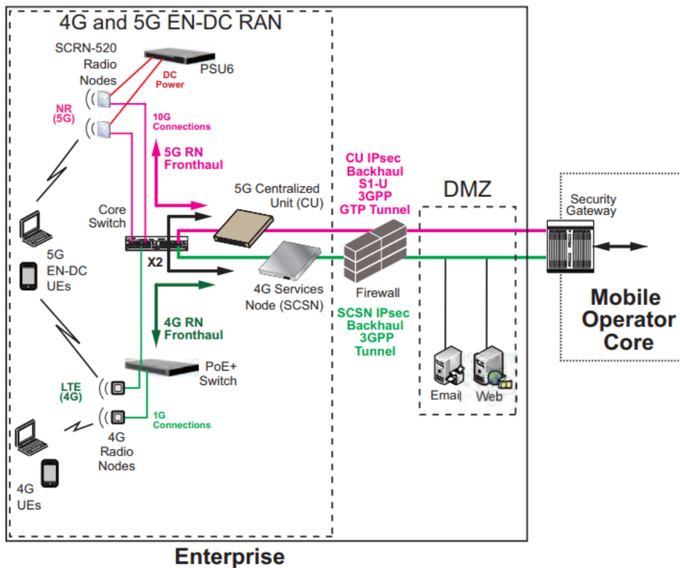
Figure 1 4G and 5G E-RAN Architecture
