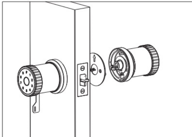
10.5: Connect the power cord between the rear panel and the front panel.
