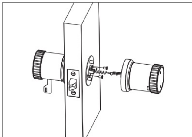
10.6: Need to keep parallel to screw on three screws, can not be crooked. Otherwise, the lock will be stuck.
