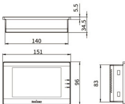
Wall mounting
