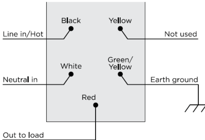
Figure 4. Single device location, with neutral connection (recommended)
