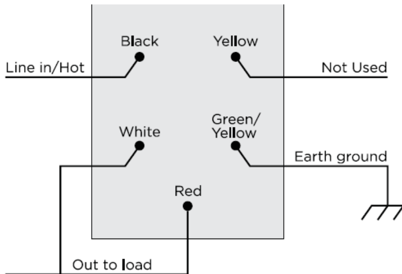
Figure 5. Single device location, without neutral connection
