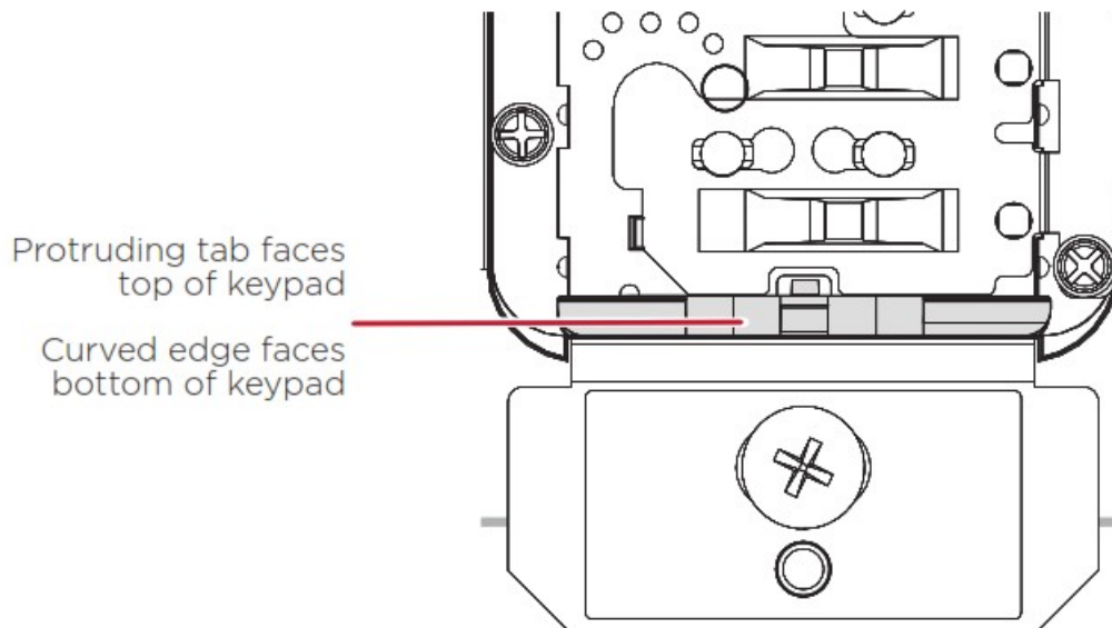
Figure 3: Attach sensor bar (shown without split up/down buttons)
