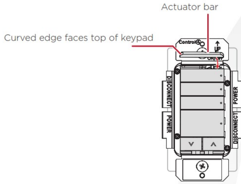
Figure 6: Attach actuator bar
