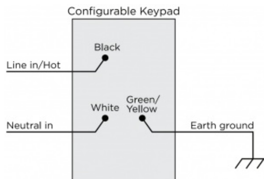
Figure 2. Keypad wiring
