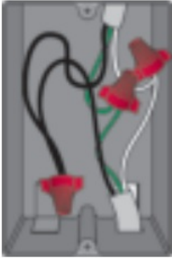
Figure 3. Bend the wires
