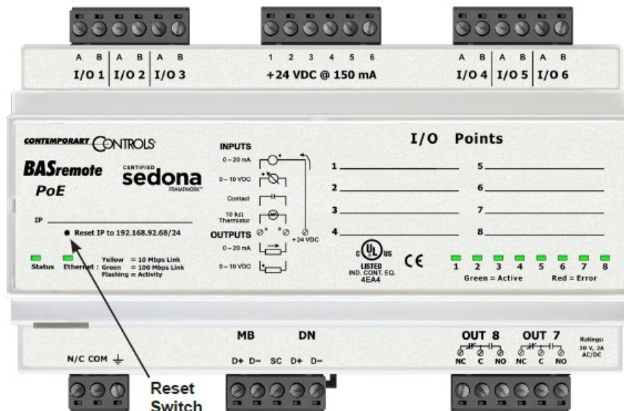
Figure 4 — BASremote PoE Image
