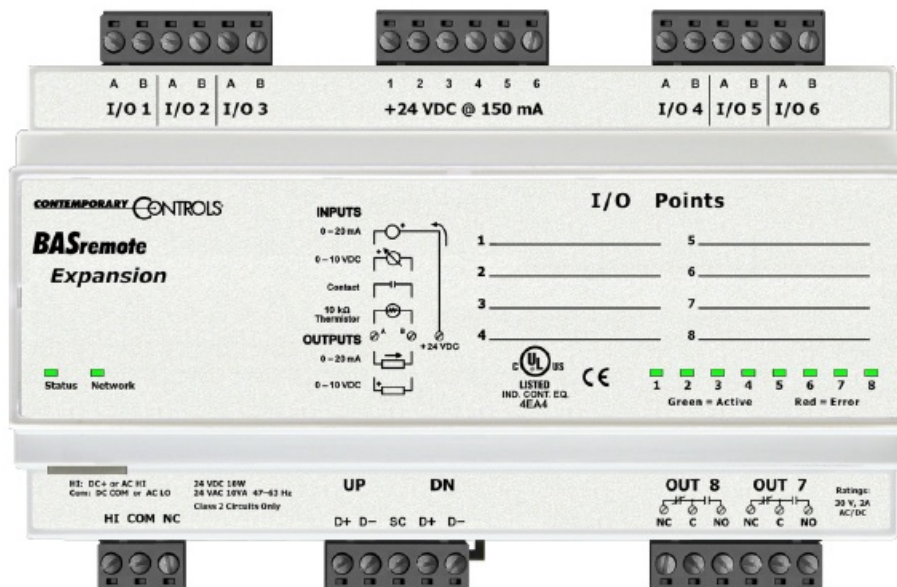
Figure 3 — BASremote Expansion Image
