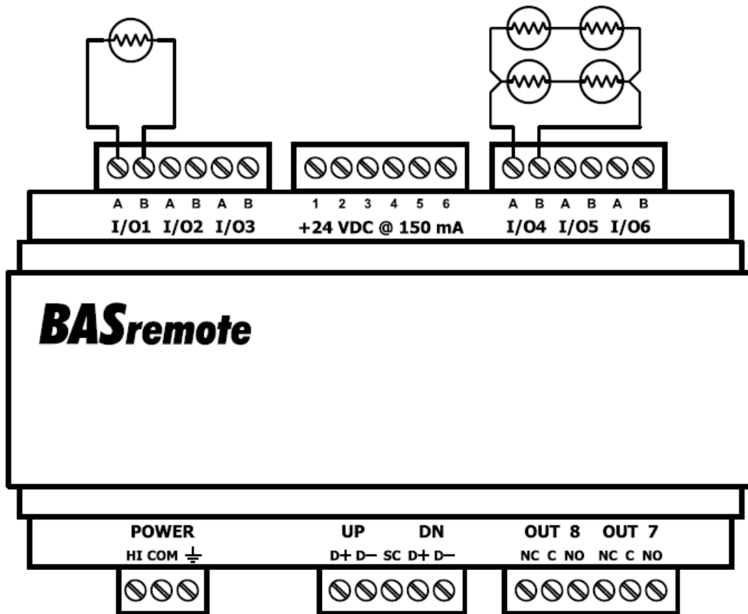
Figure 11 — Thermistor Connections
