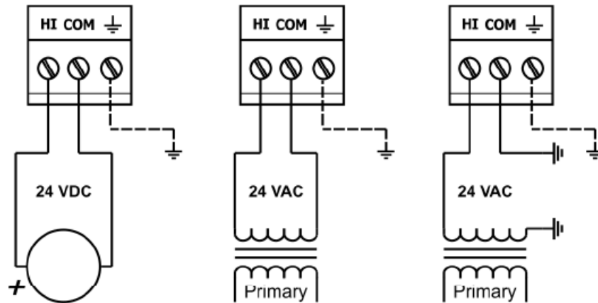
Figure 8 — Power Options
