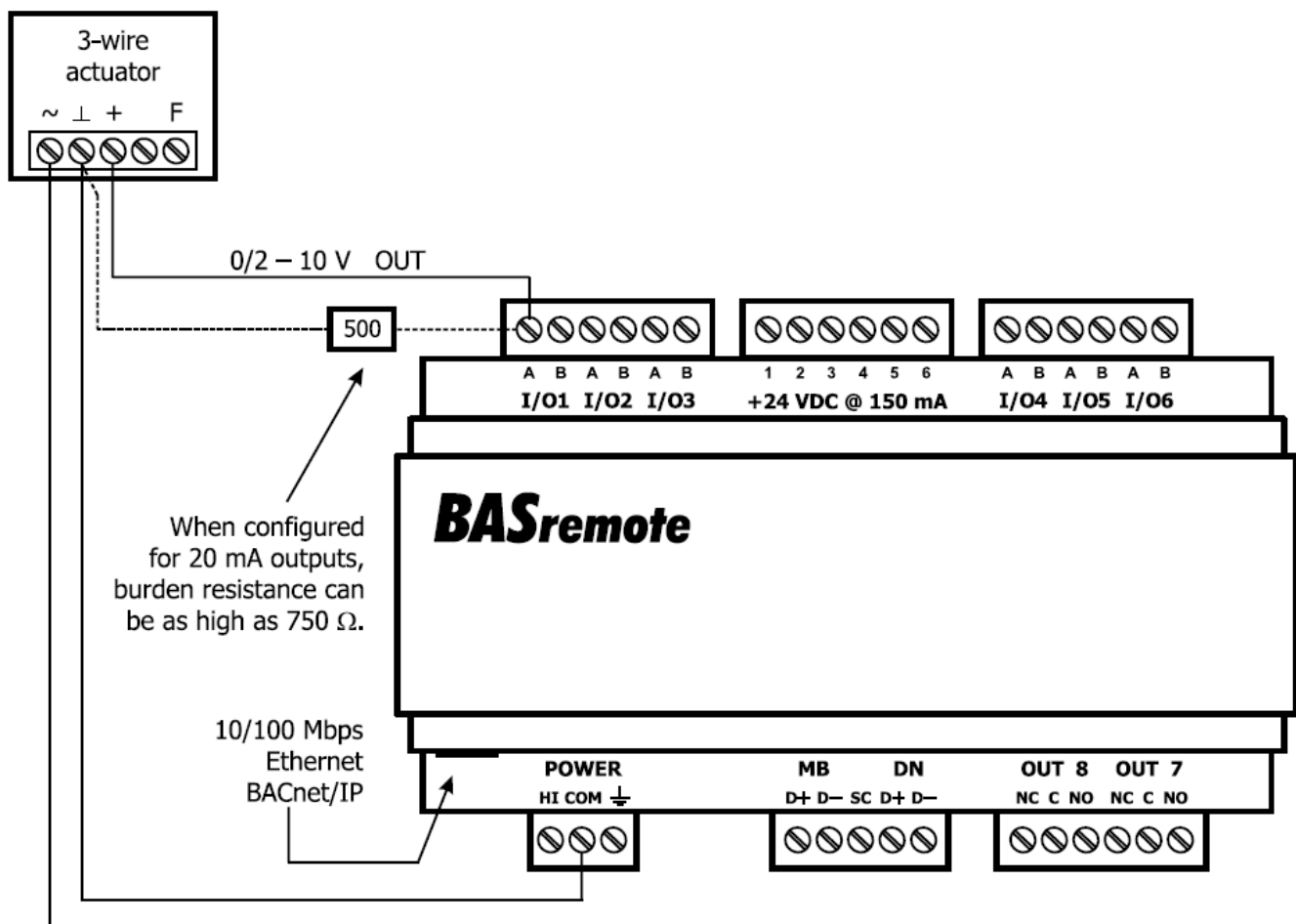
Figure 15 — Analog Output Connections
