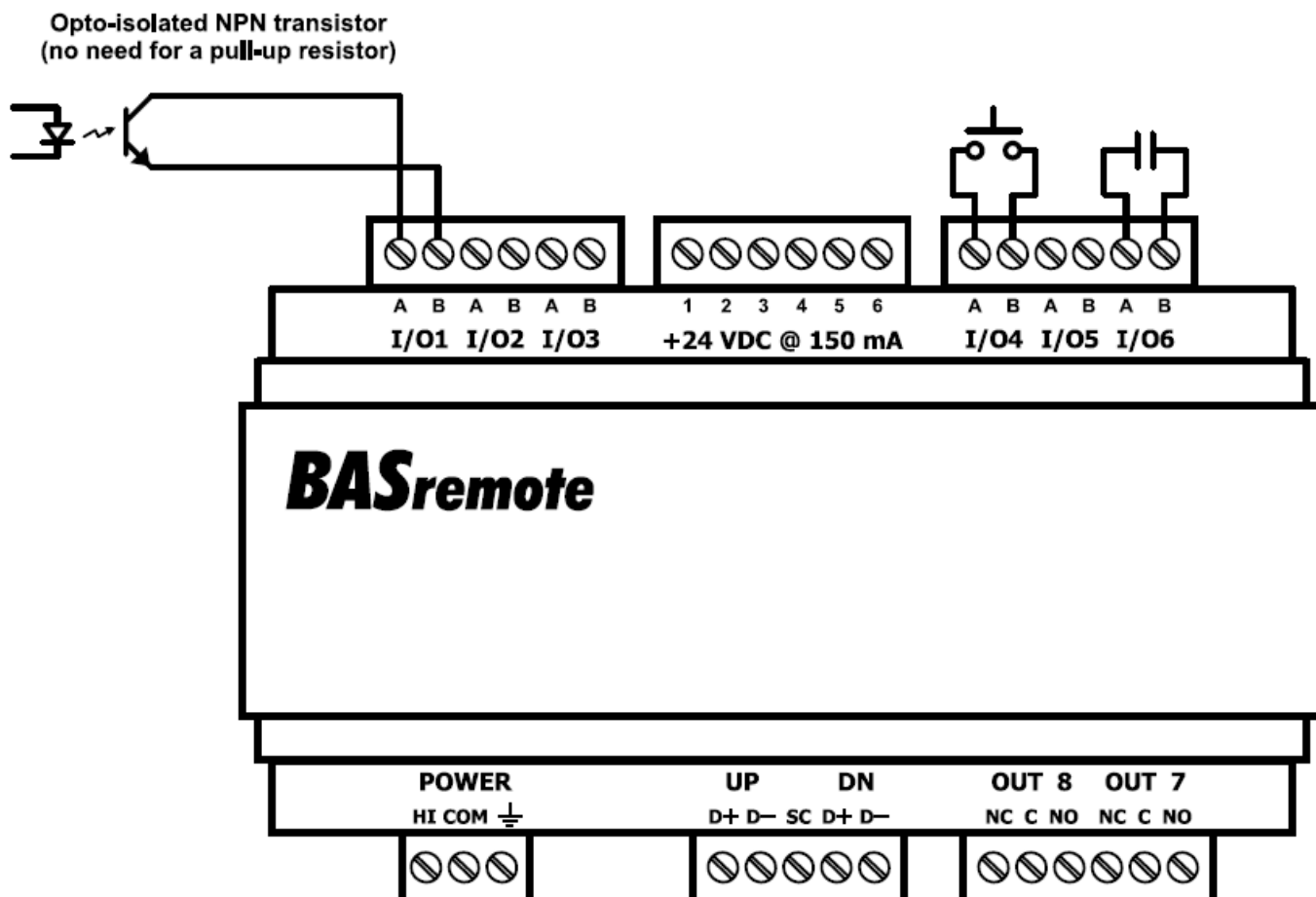
Figure 12 — Contact Closure Connections
