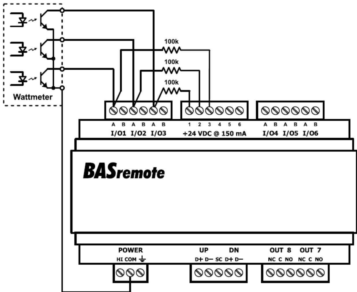
Figure 13 — Pulse Input Connections
