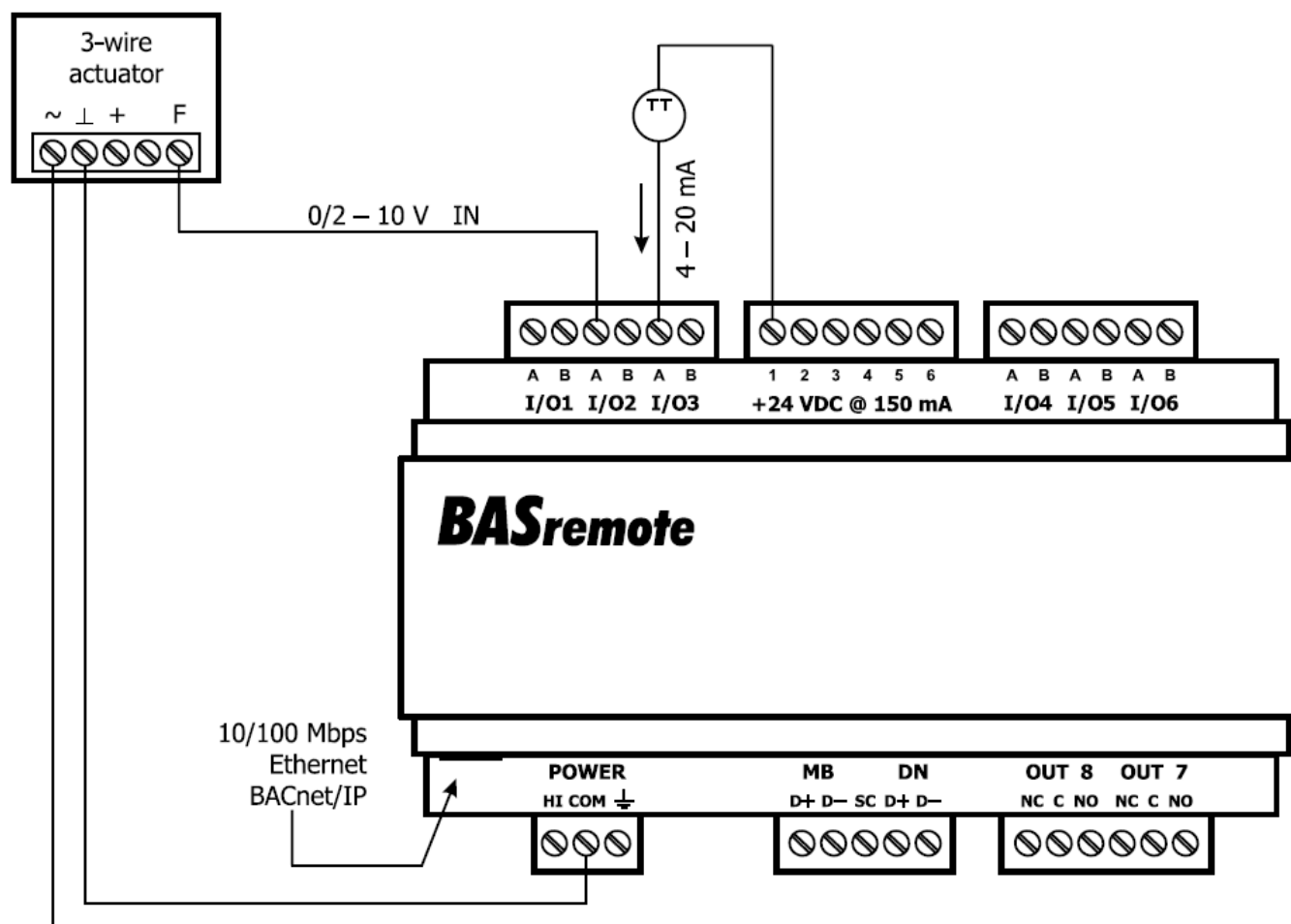
Figure 14 — Analog Input Connections
