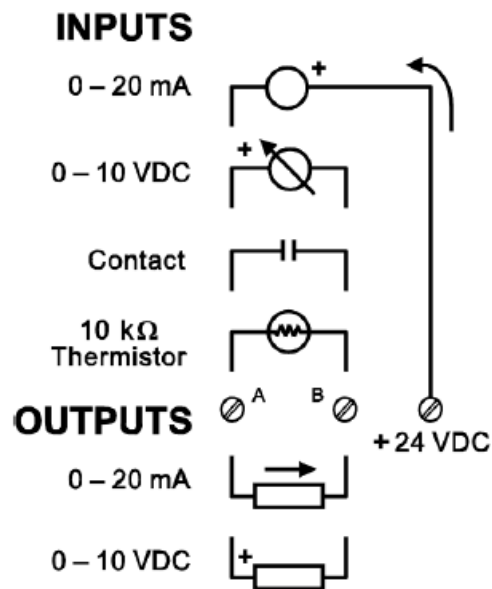
Figure 10 — I/O Options (Channels 1–6)
