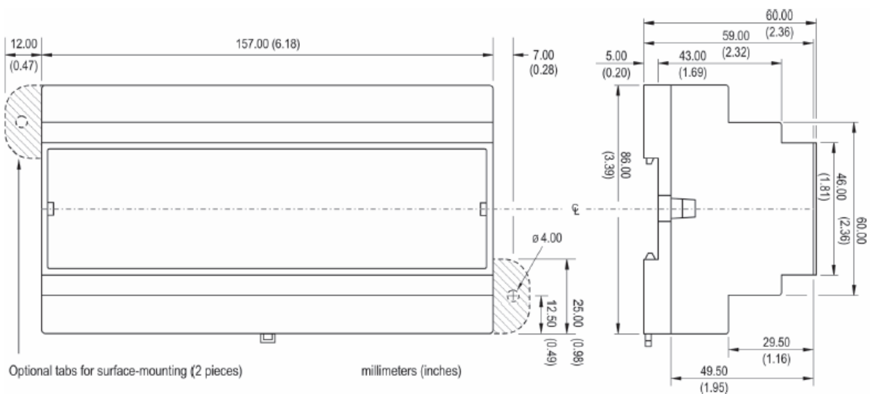
Figure 5 — BASremote Dimensional Drawing for All Models
