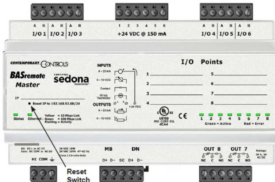
Figure 2 — BASremote Master Image
