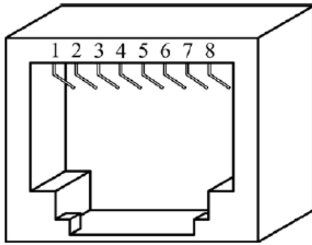
Figure 1 — RJ-45 Jack
