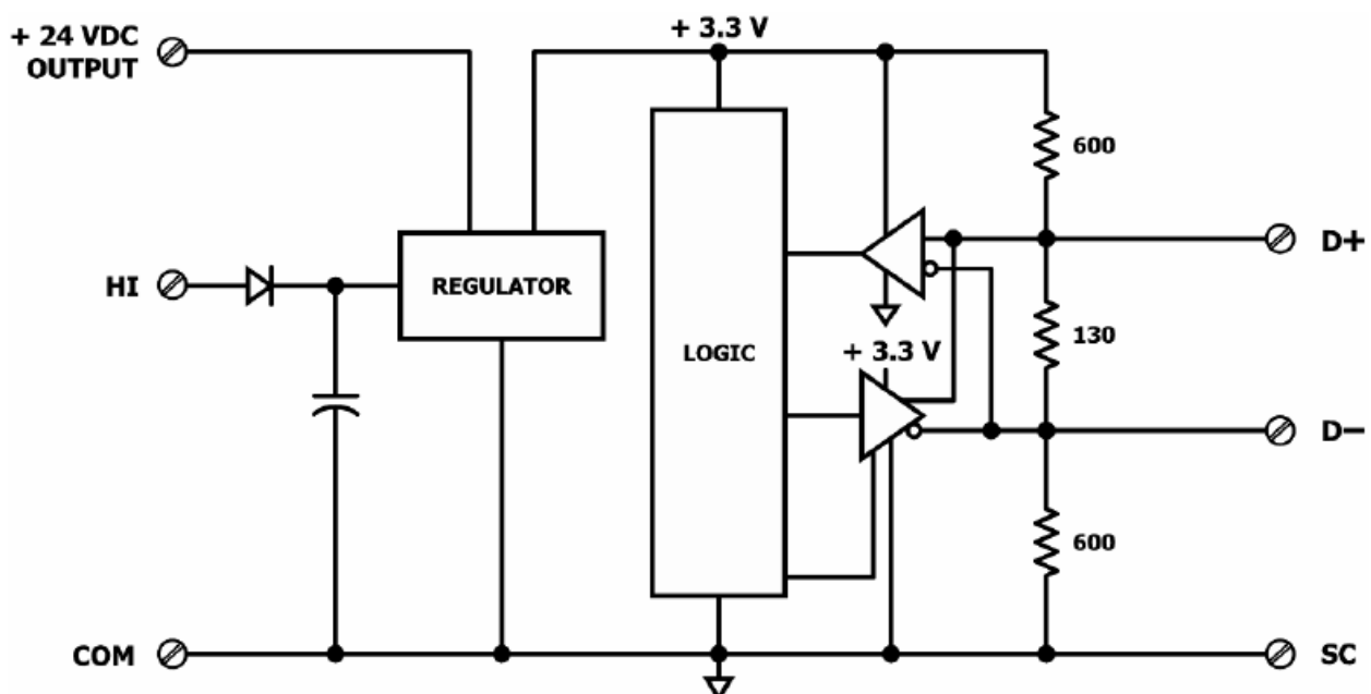
Figure 7 — Internal Termination and Bias
