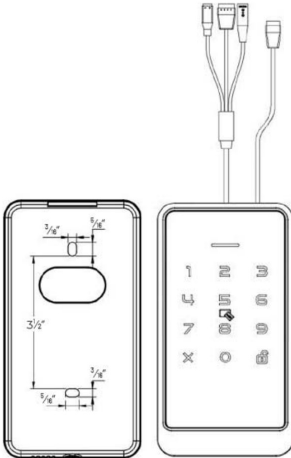
Access Panel Specifications
