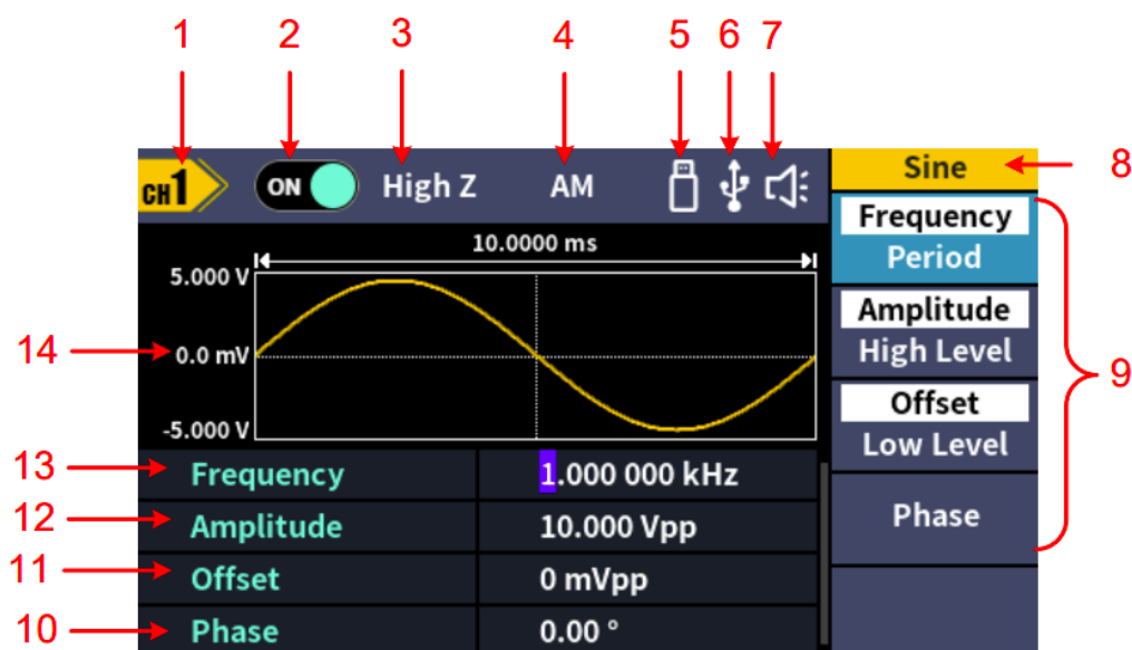
Figure 4-3 User Interface
