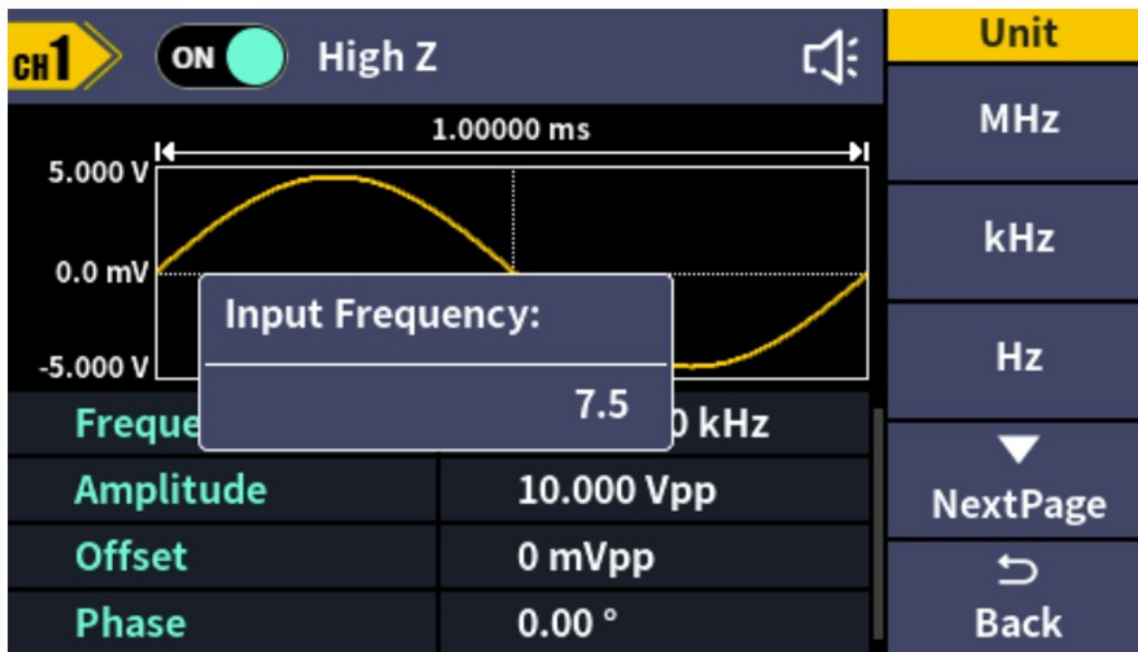
Figure 4-4 Use numeric keypad to set the frequency
