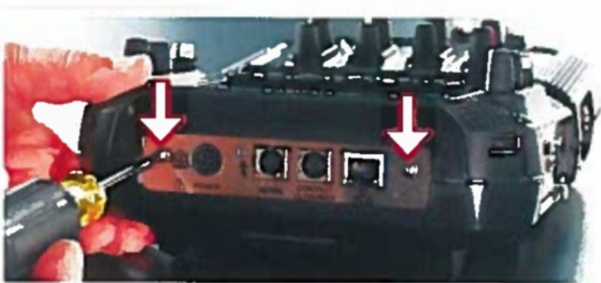
Figure 5 – Mounting Screws
