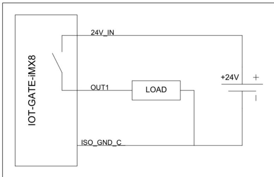
Figure 3 Digital output – typical wiring example
