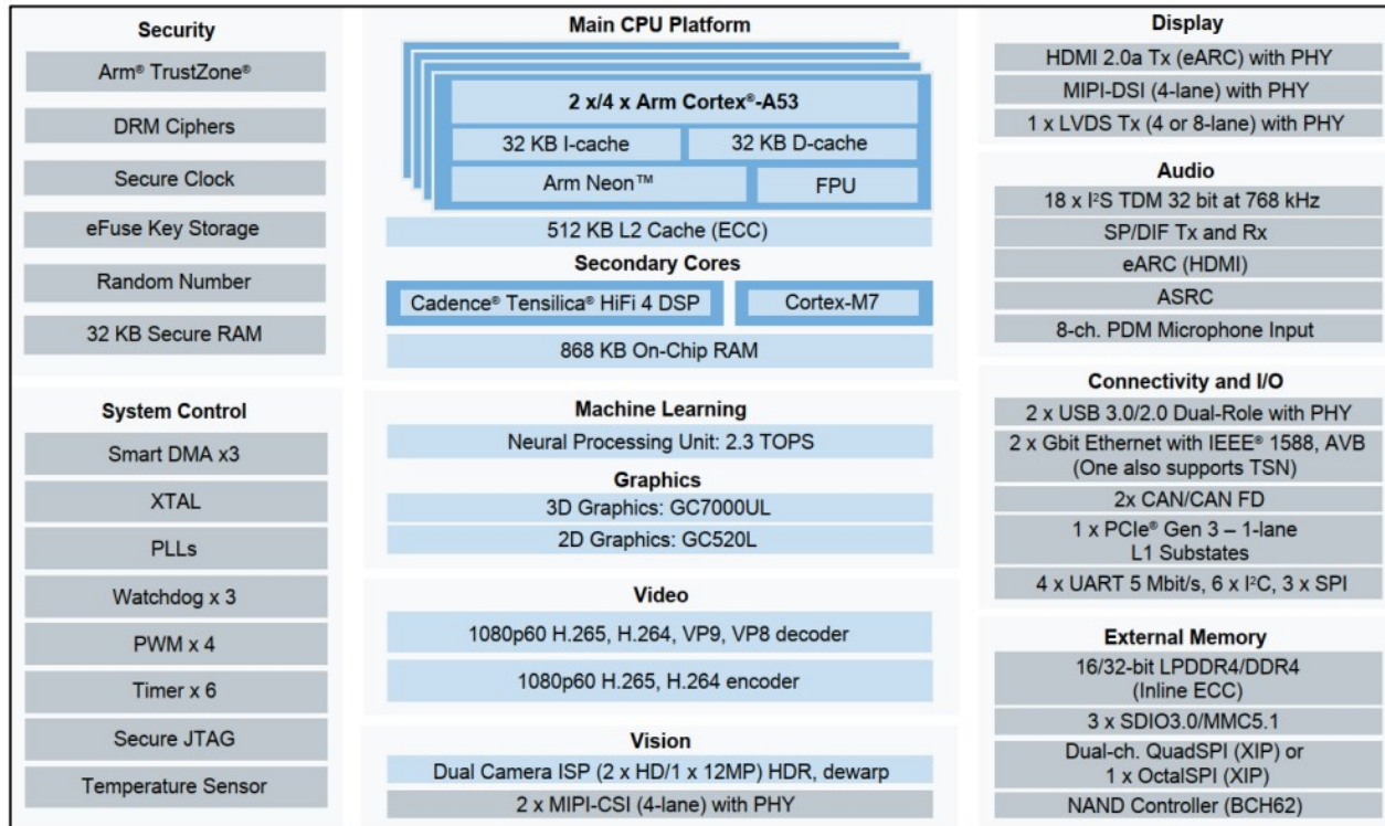
Figure 1 i.MX8M Plus Block Diagram
