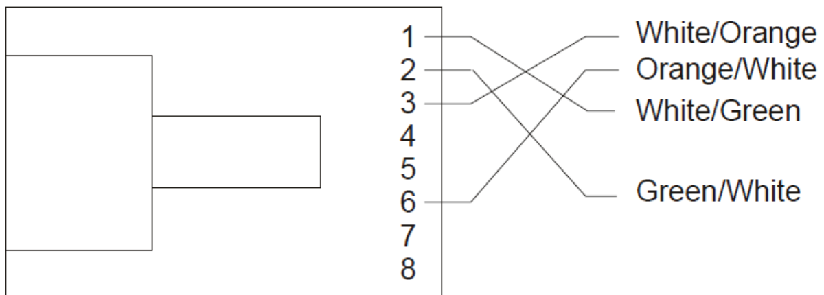
Figure C-2. 10/100 external crossover for RJ-45 connector
