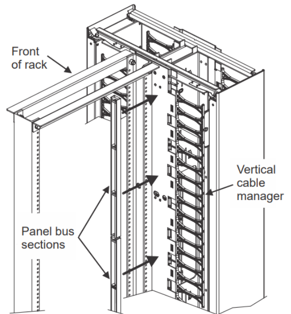
Panel Bus Mounting on Side of Vertical Cable Manager
