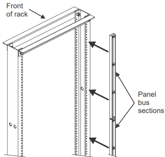
Panel Bus Mounting on Rear Flange of Rack
