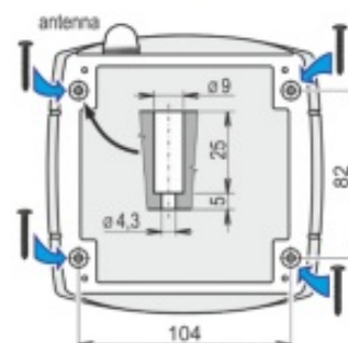
Device mounting
