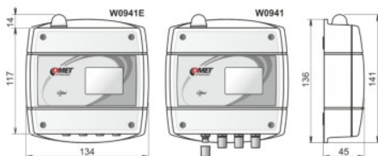
Dimensions (mm)
