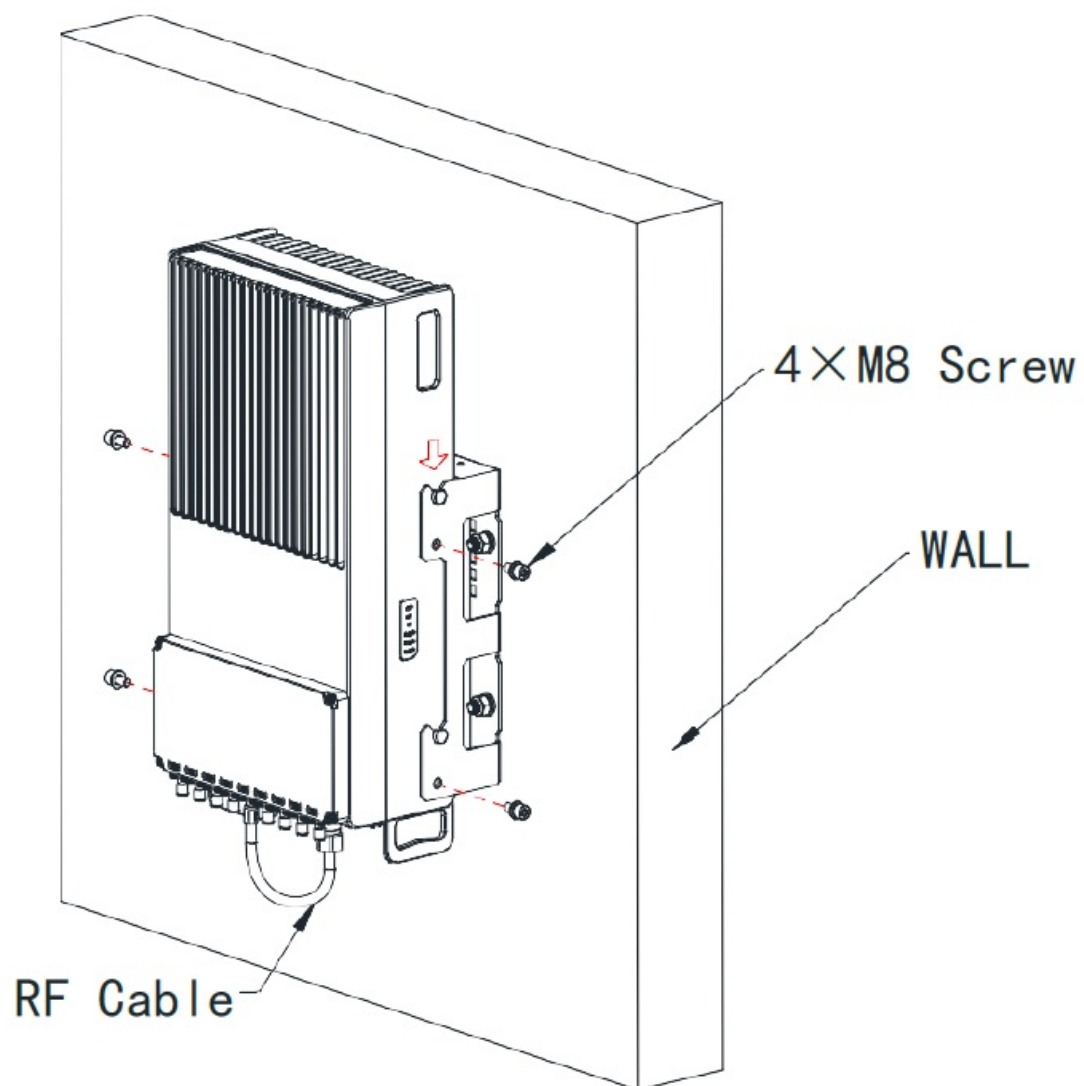
Figure 7 Wall Mounting (with Splitter)
