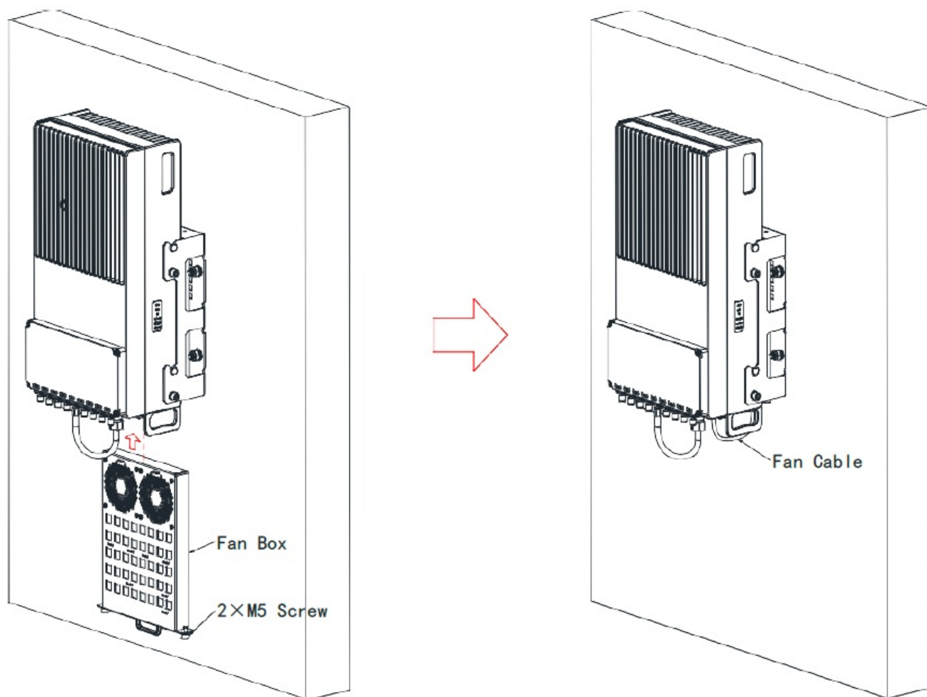
Figure 8 Fan Installation
