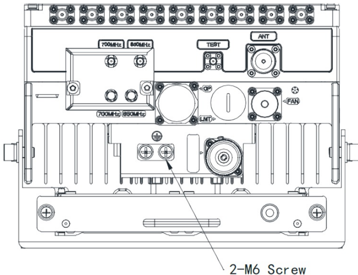
Figure 9 Grounding Cable Diagram
