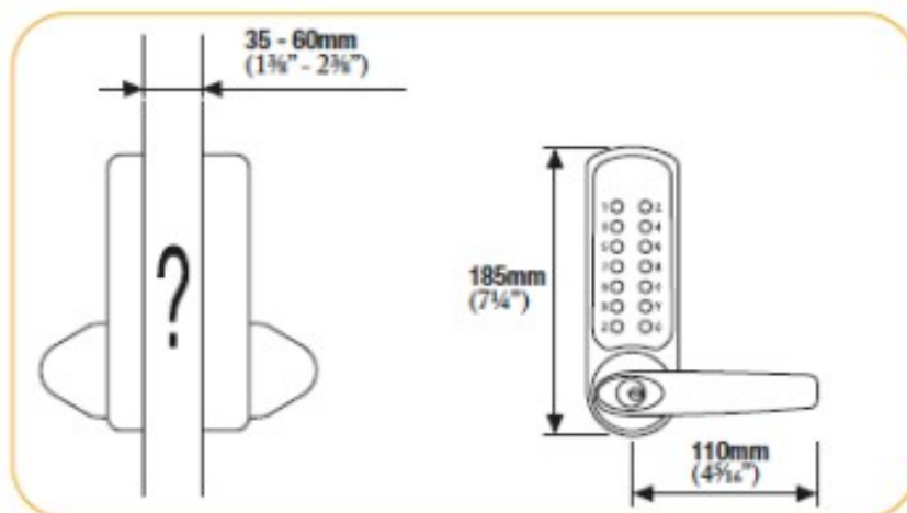
Model 600/605 For use with existing lock
