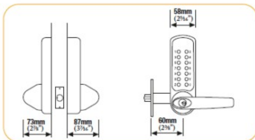
Model 610/615 With tubular latchbolt
