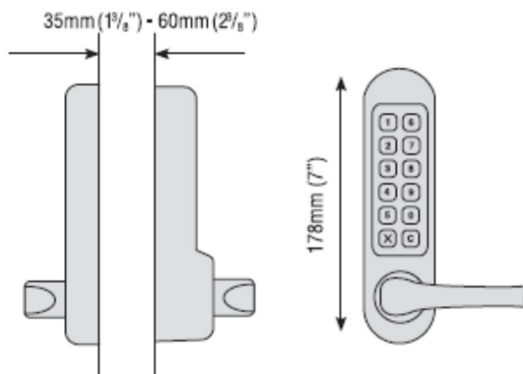
CL500/CL505 for use with existing lock
