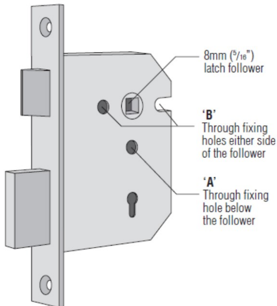
FIGURE 1- LOCK CASE
