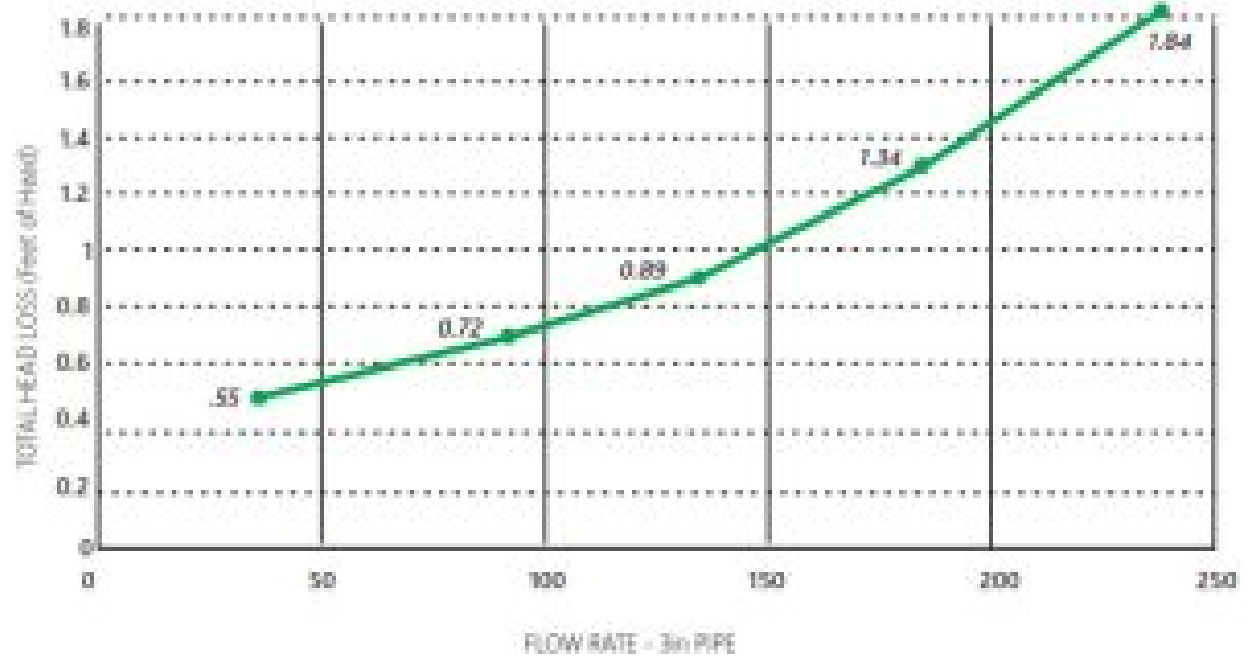
HEAD LOSS CHARTS
