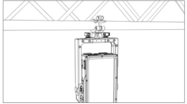
f. Yoke 2.2 with 1x Omega Bracket
