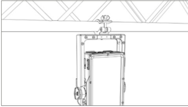
e. Yoke 2.2 with 1x Mounting Clamp
