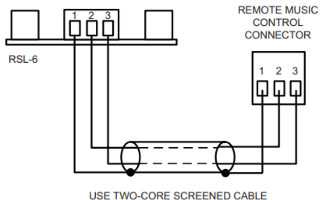
REMOTE SOURCE & LEVEL CONTROL WIRING
