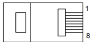
RJ-45 PLUG (PIN SIDE)
