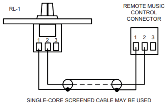
REMOTE LEVEL CONTROL WIRING
