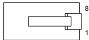
RJ-45 PLUG (LATCH SIDE)
