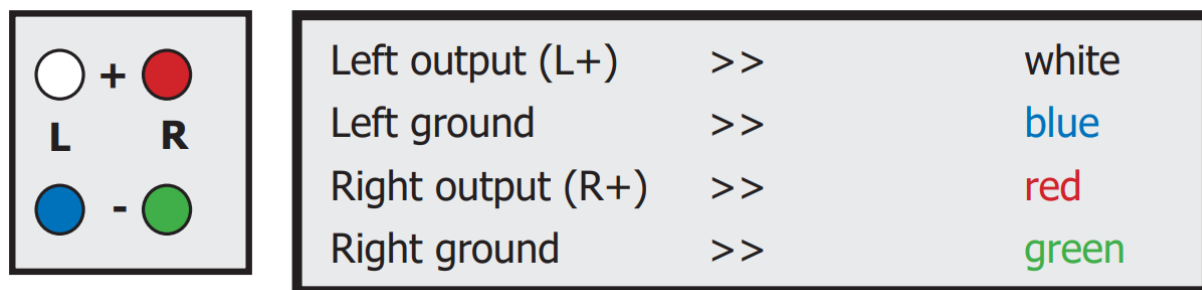
Pic. 1: Colour marking of the signal pins
