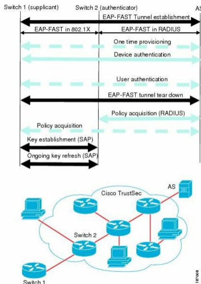
Figure 2: Cisco TrustSec Authentication
