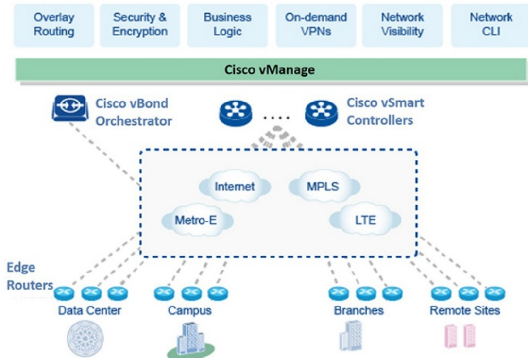
Figure 6: Components of Cisco Catalyst SD-WAN
