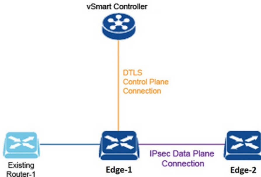
Figure 7: An Edge Router Placed into an Existing Network
