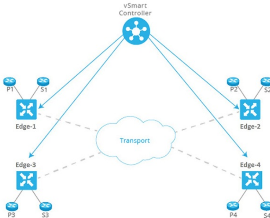
Figure 1: Components of the Cisco Catalyst SD-WAN Solution
