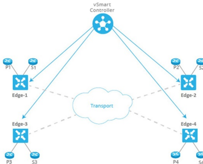
Figure 3: Centralizing Routing Intelligence with a Centralized Controller
