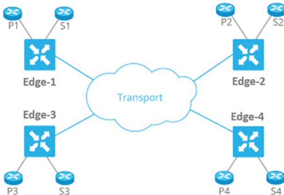
Figure 2: Transport Network Separated from Service Network
