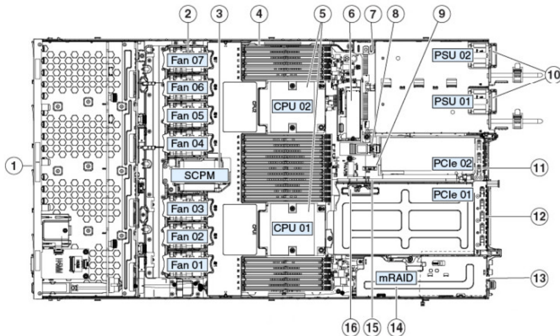
Figure 6: Serviceable Component Locations
