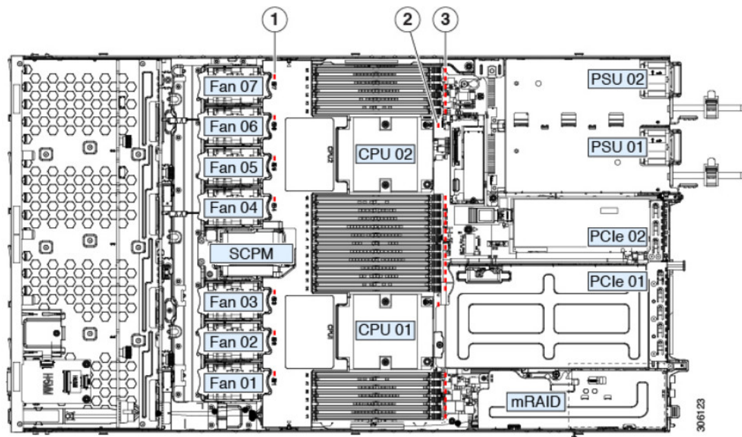
Figure 5: Internal Diagnostic LED Locations
