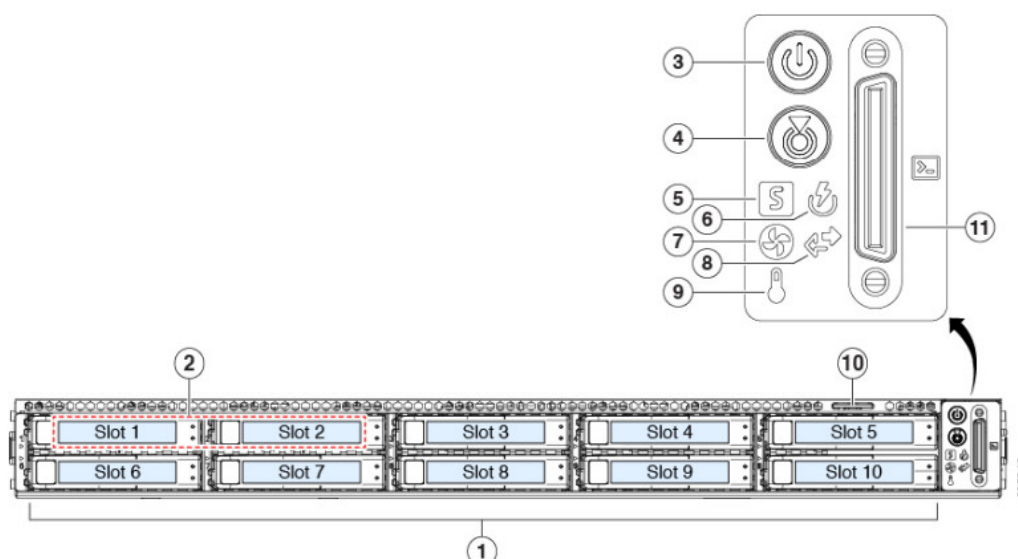
Figure 1: Cisco SNS 3600 Series Appliance Front Panel
