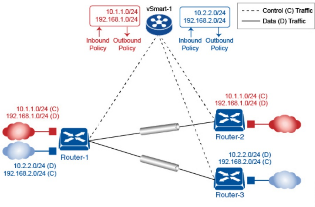
Figure 1: Propagation of Routing Information Inside a VRF
