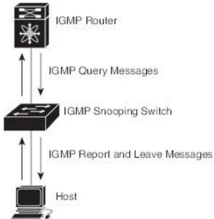
Figure 1: IGMP Snooping Switch
