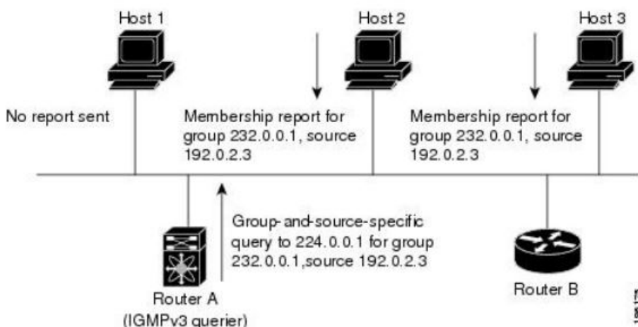
Figure 2: IGMPv3 Group-and-Source-Specific Query
