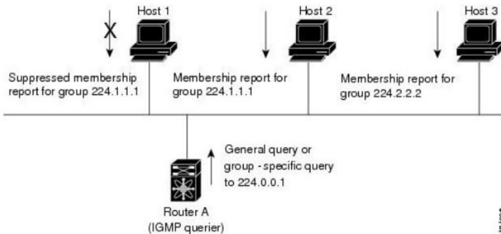
Figure 1: IGMPv1 and IGMPv2 Query-Response Process
