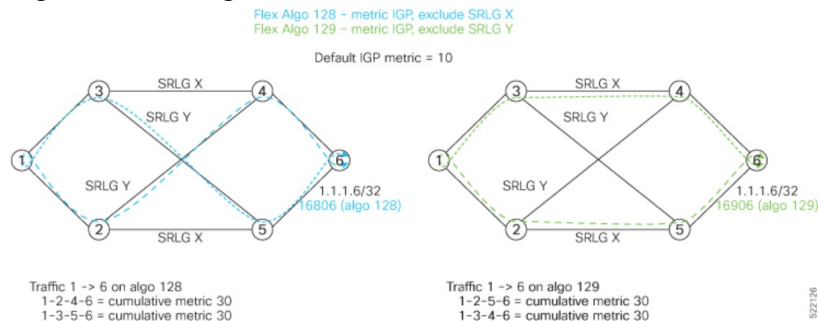
Figure 1: Flex Algo with Exclude SRLG Constraint
