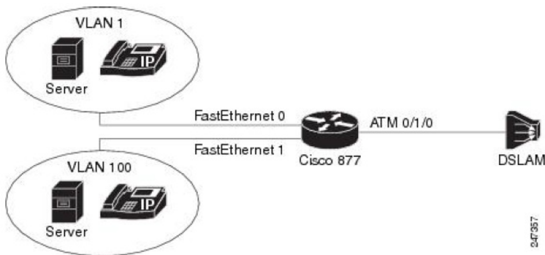
Figure 1: VLAN-Based Service Differentiation at PVC Level
