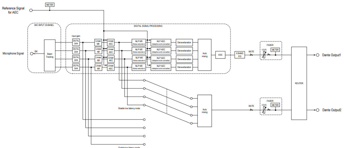
Figure 2: RM-CG internal components, Dante input and outputs
