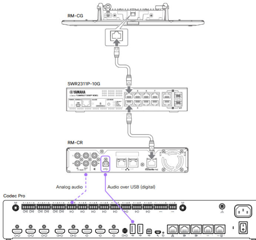
Figure 1: Connecting audio input components via USB
