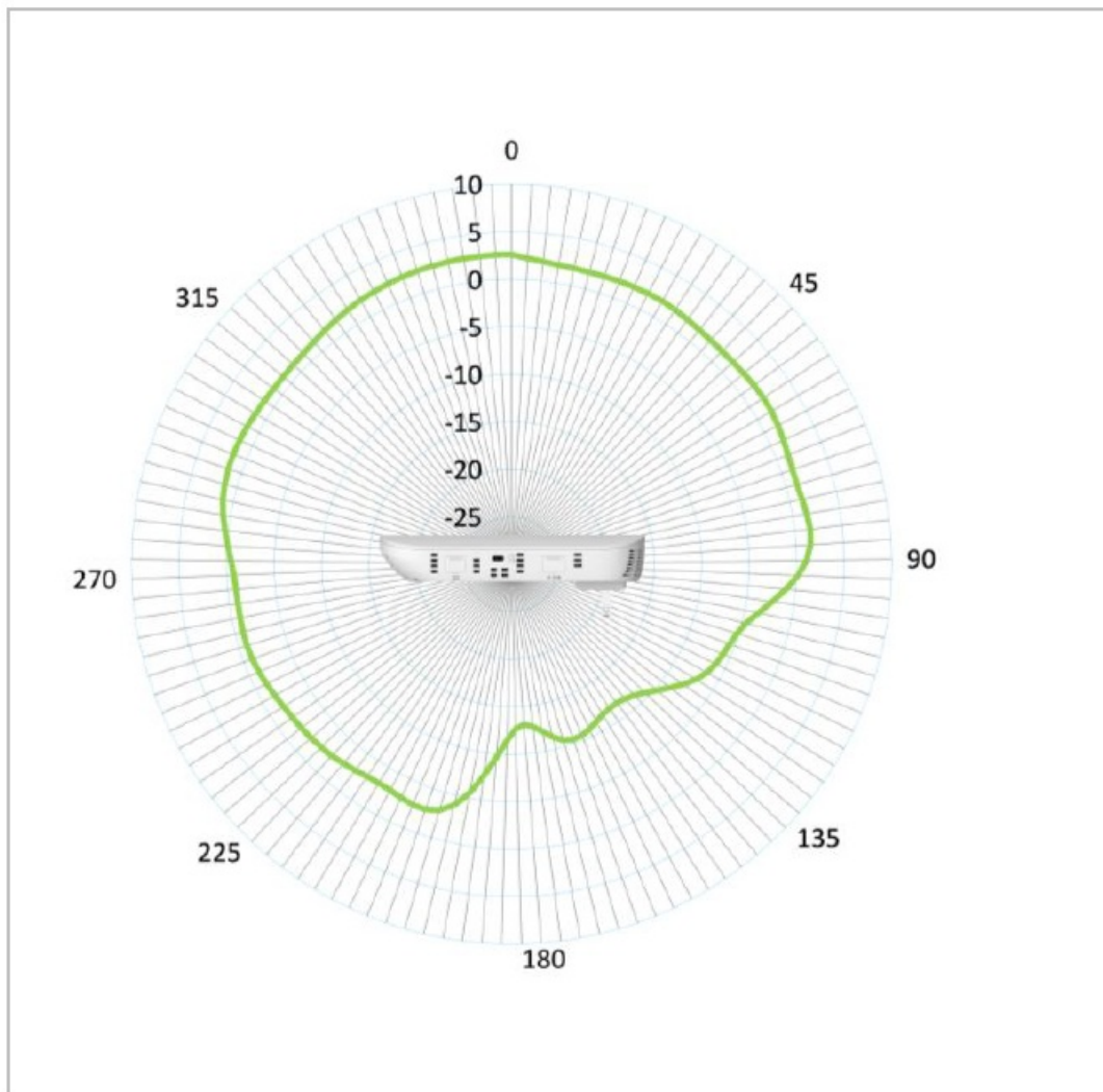
Figure 3. Cisco CBW151AX Antenna Pattern 2.4GHz Elevation
