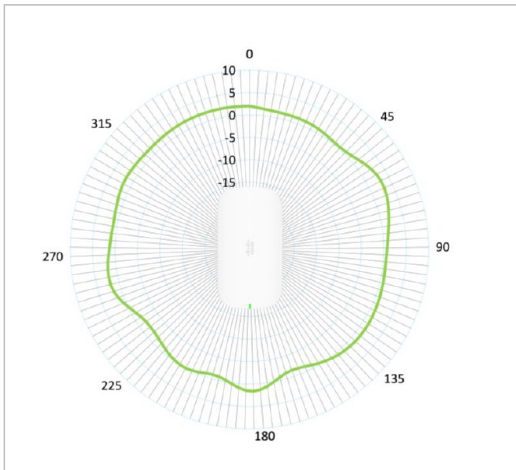
Figure 4. Cisco CBW151AX Antenna Pattern 5GHz Azimuth
