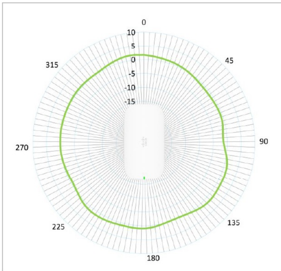
Figure 2. Cisco CBW151AX Antenna Pattern 2.4GHz Azimuth
