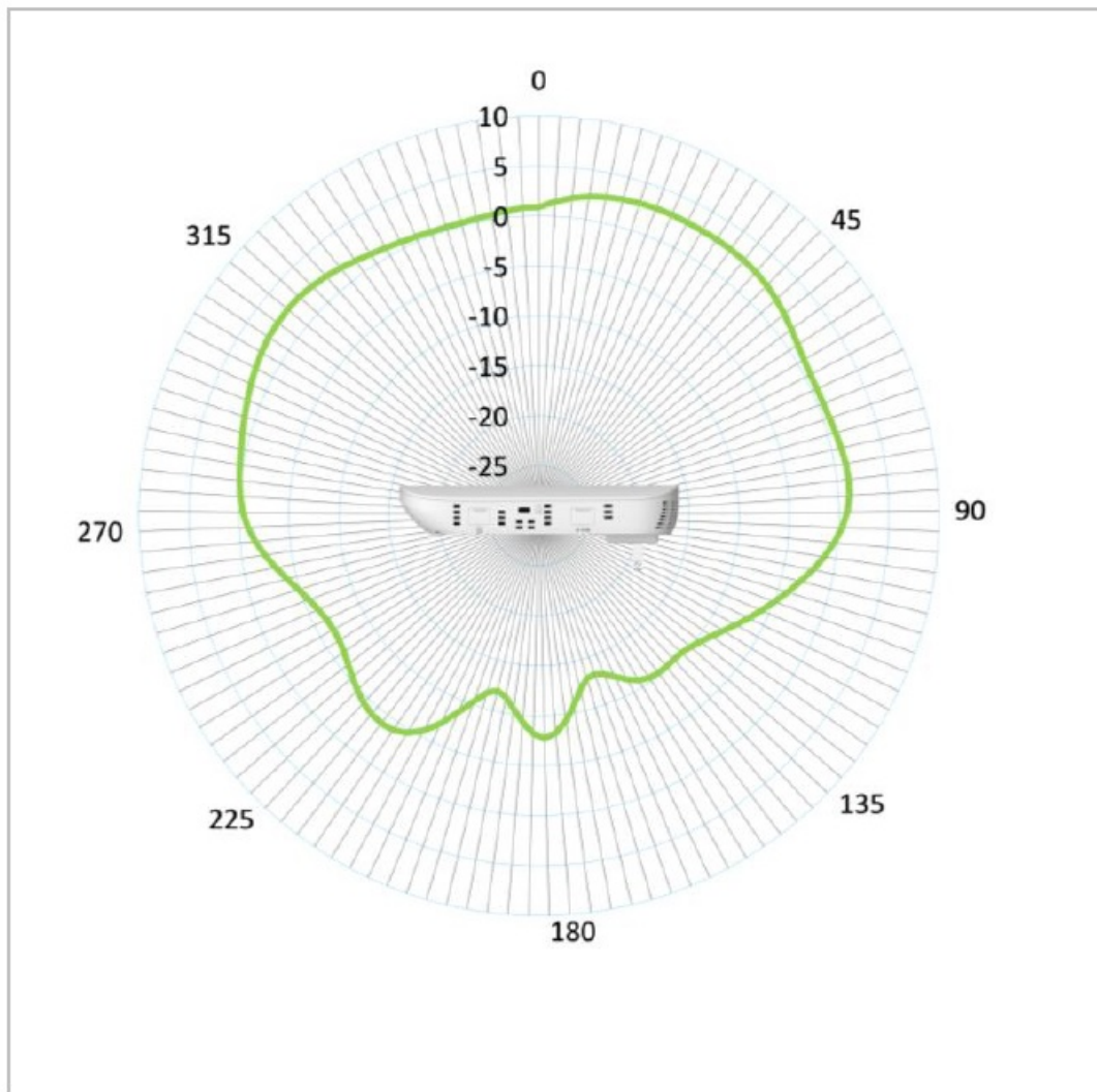
Figure 5. Cisco CBW151AX Antenna Pattern 5GHz Elevation
