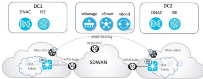
Figure 3: Solution Test Multicast Topology
