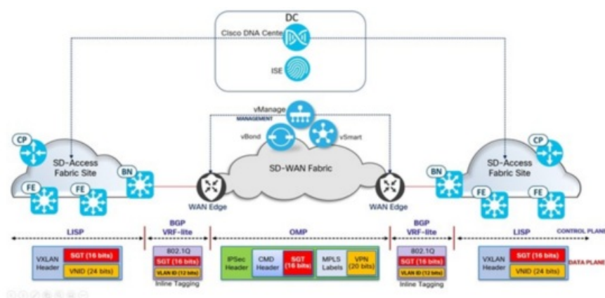
Figure 2: SD-Access SD-WAN Integration with Inline SGT
