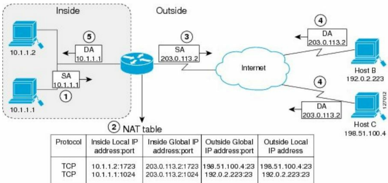
Figure 2: NAT Overloading Inside Global Addresses
