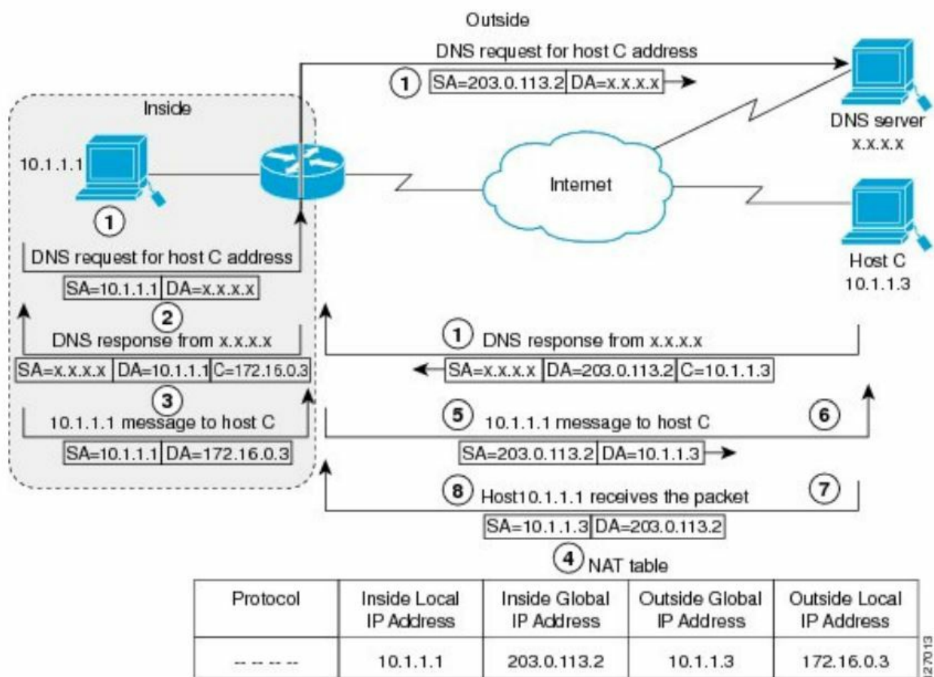
Figure 3: NAT Translating Overlapping Addresses
