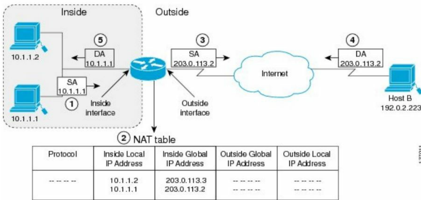
Figure 1: NAT Inside Source Translation
