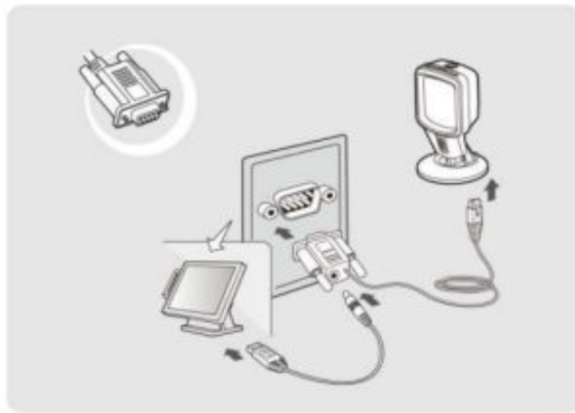
RS232 Serial
