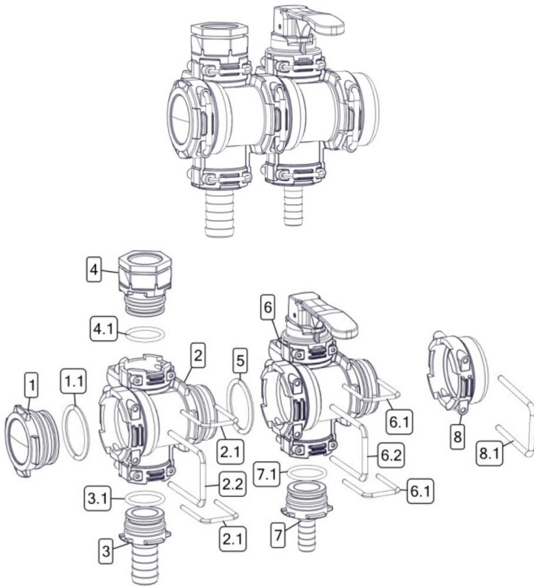
ARAG NPT+1 Two Sec Valve Assembly #5282495
