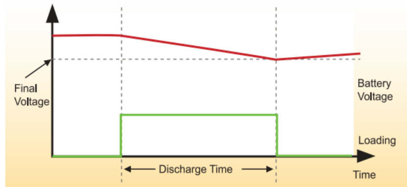
Figure 5 : Battery Discharge Testing
