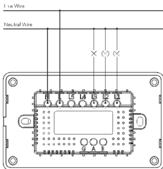
Live & Neutral wire (Neutral wire Required )
