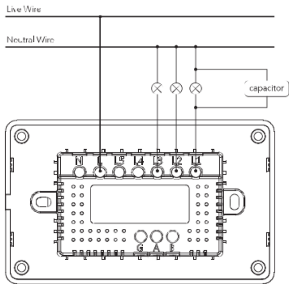
Single Live Wire (No Neutral Wire Required )
