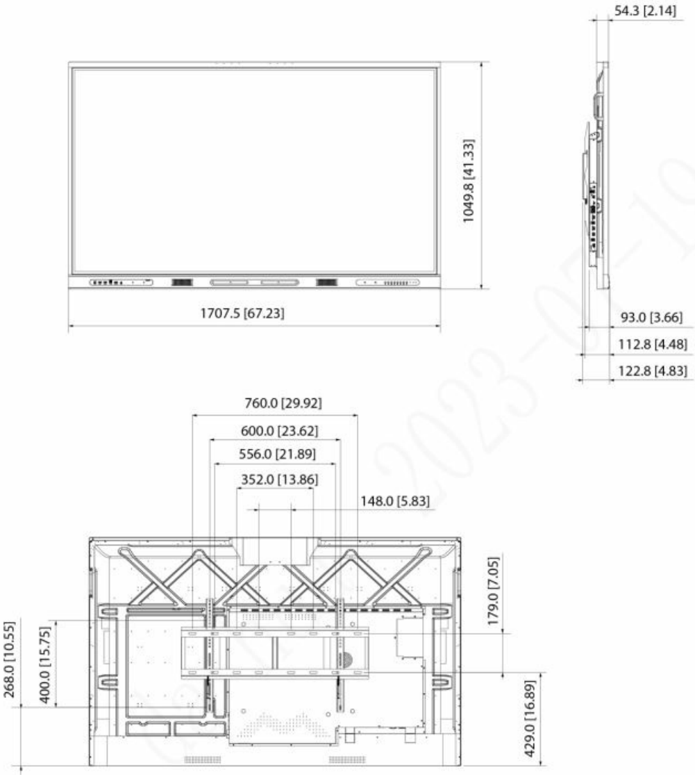
Figure 1-6 Dimensions (without camera) (mm[inch])
