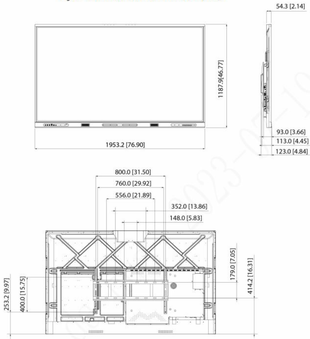
Figure 1-8 Dimensions (without camera) (mm[inch])
