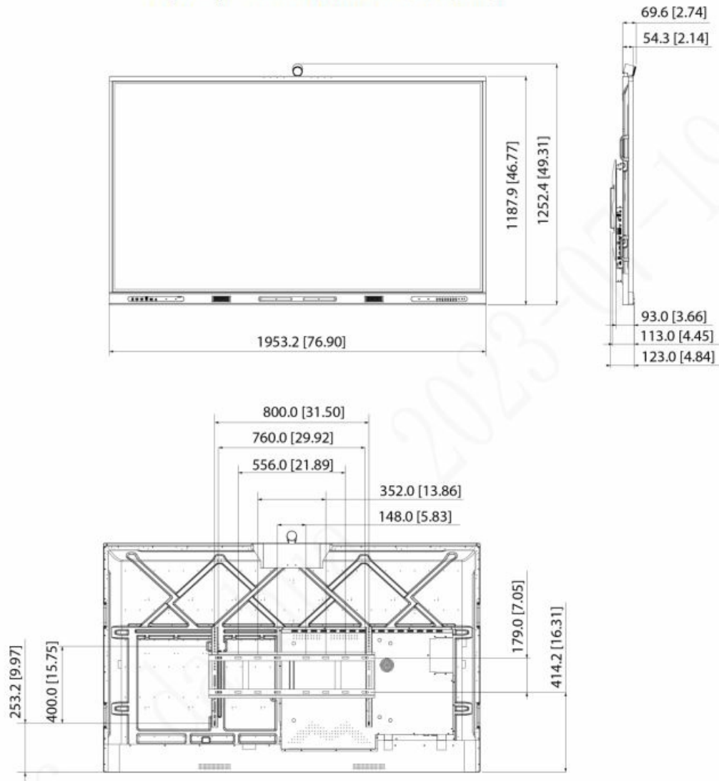
Figure 1-7 Dimensions (with camera) (mm[inch])
