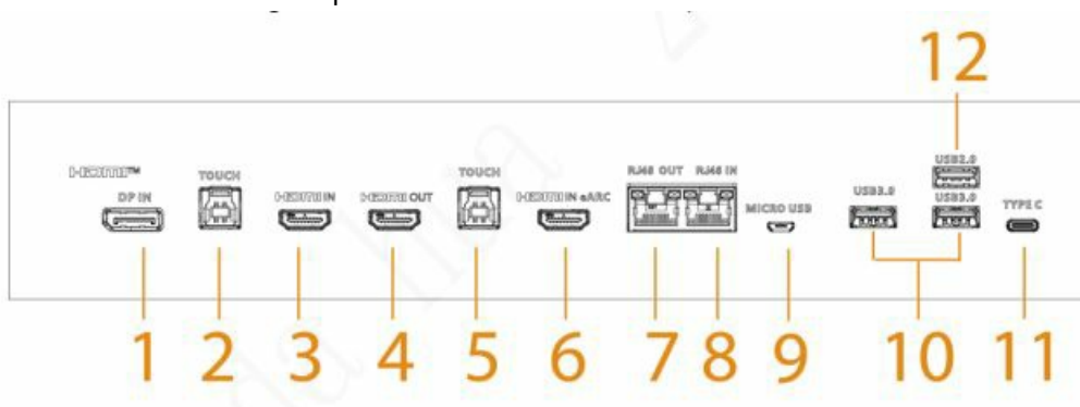
Figure 1-10 Ports on the side of the rear panel
