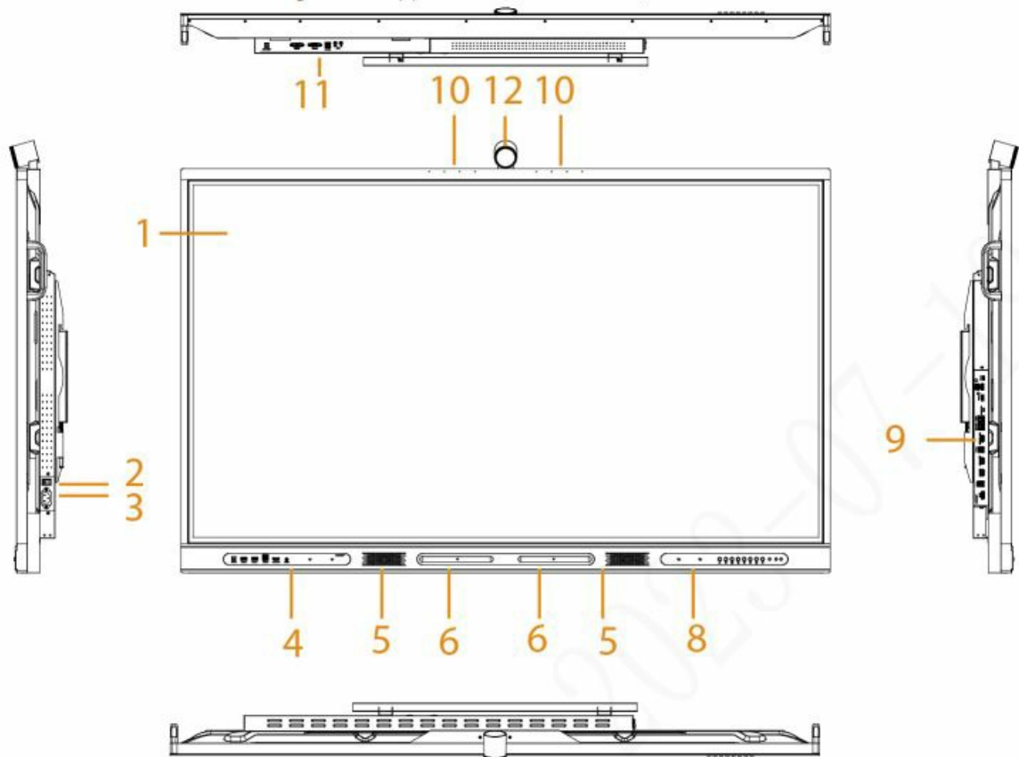
Figure 1-1 Appearance (with camera)
