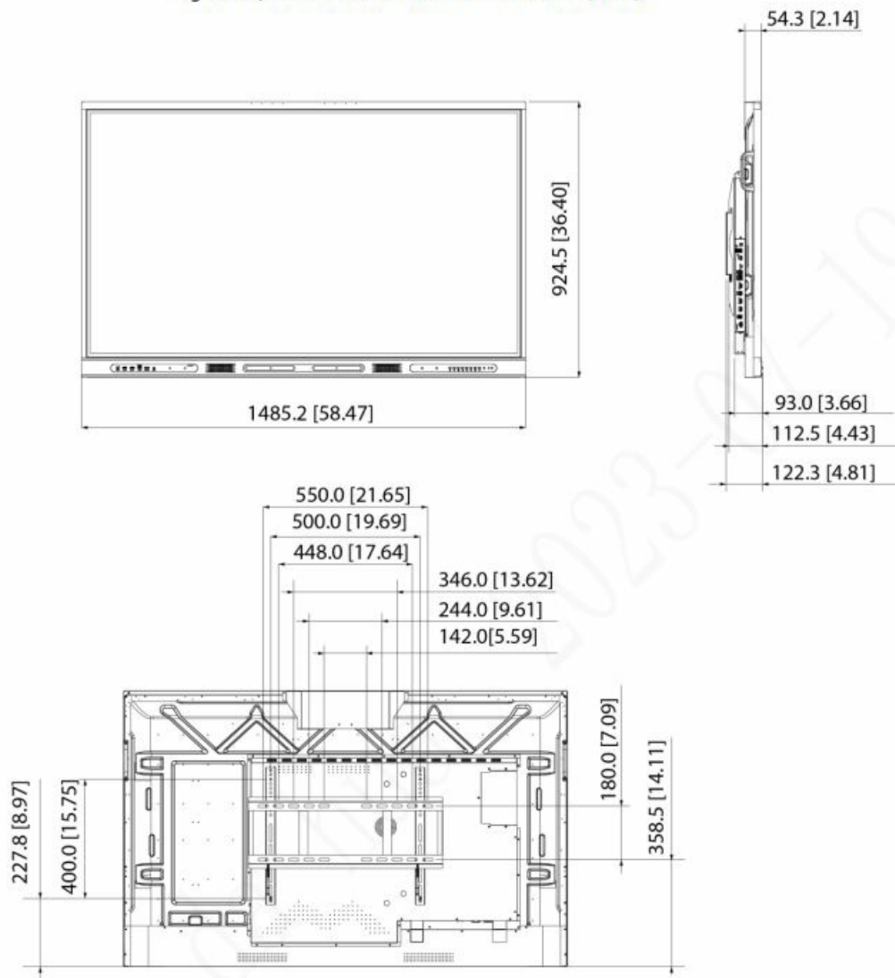
Figure 1-4 Dimensions (without camera) (mm [inch])
