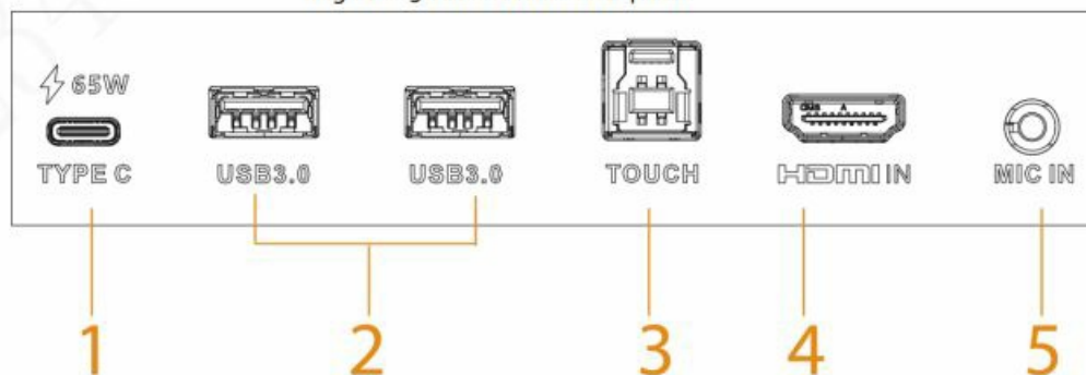
Figure 1-9 Ports on the front panel
