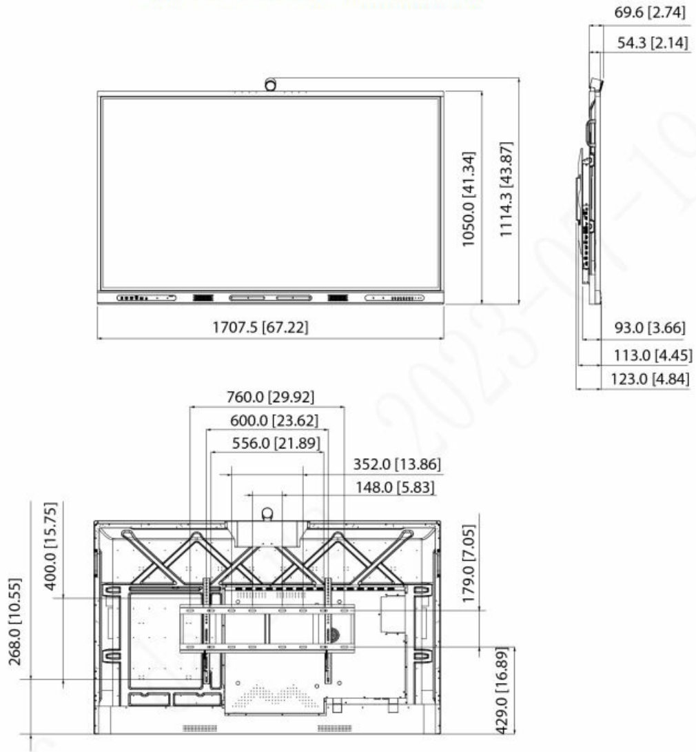
Figure 1-5 Dimensions (with camera) (mm[inch])
