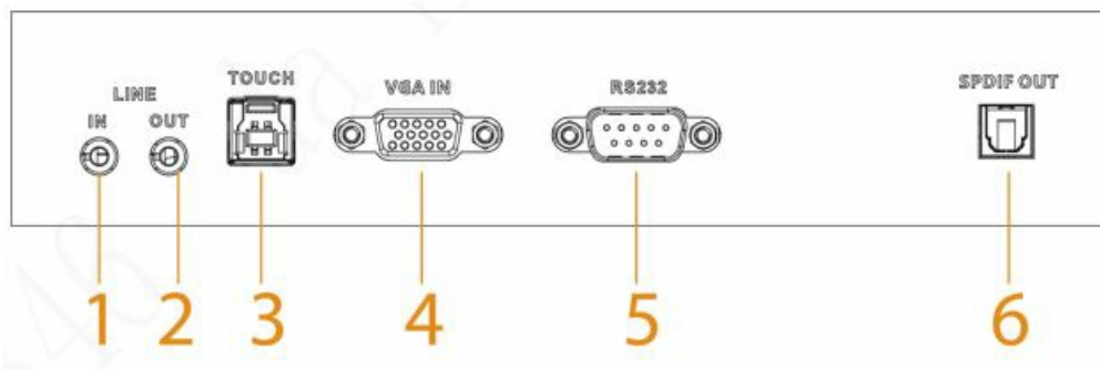
Figure 1-11 Ports on the bottom of the rear panel
